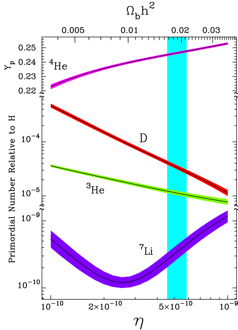
Figure 3.2: Predicted abundances of {}^4\text{He} (mass fraction), \text{D} , {}^3\text{He} and {}^7\text{Li} (number relative to hydrogen) as a function of the baryon-to-photon ratio \eta and the baryon density parameter \Omega_{\text{B}}h^2 [?]. The shadow band embedding each curve indicates 2\sigma theoretical uncertainty. The dark band shows the determination of the baryon density based upon the recent measurement of the primordial abundance of deuterium, \Omega_{\text{B}}h^2 = 0.019 \pm 0.0024 [?]. The baryon density \rho_{\text{B}} is calculated by the baryon-to-photon ratio \eta [?].
