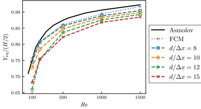
Figure 3.9 – Equilibrium position Y_{eq} of a sphere in a laminar parallel channel flow. Asmolov reference values are taken from [109]. FCM results are found in [110]
