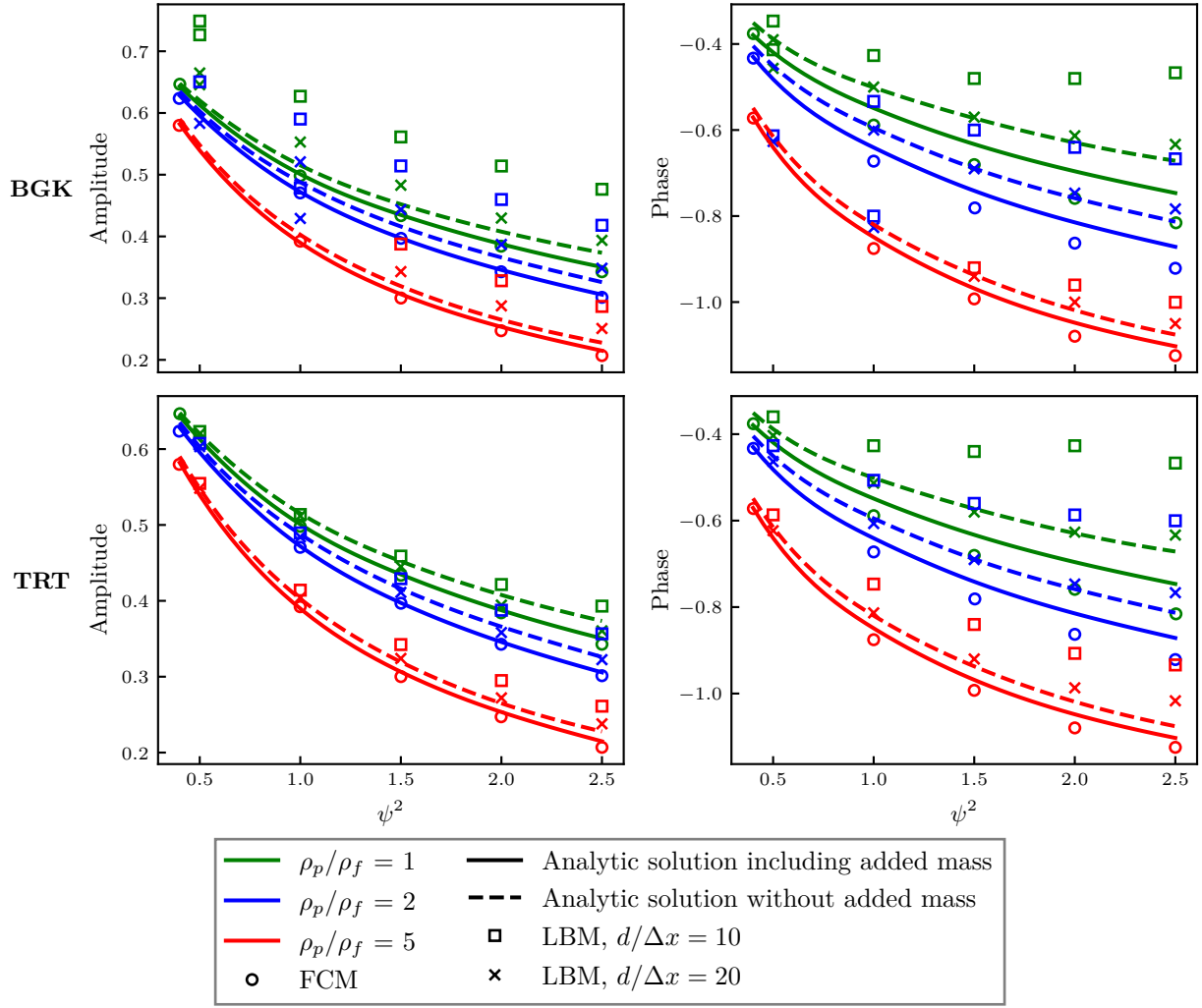
Figure 3.7 – Amplitude and phase shift of external force to particle velocity. \psi^2 = \omega d^2/\nu is the dimensionless frequency. The resolution is given by the number of lattice cells per particle diameter d/\Delta x .
