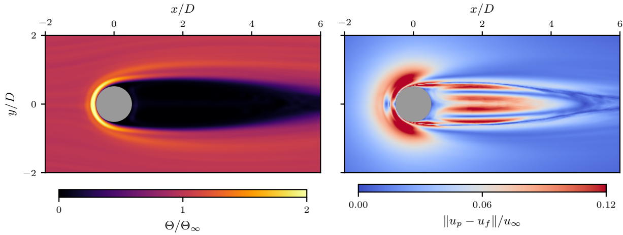
Figure 5.11 – Time averaged flow field of solid volume fraction and slip velocity of a suspension with iron particles, \Theta_\infty = 0.1 and \text{Re}_{\text{eff}} = 64 .
