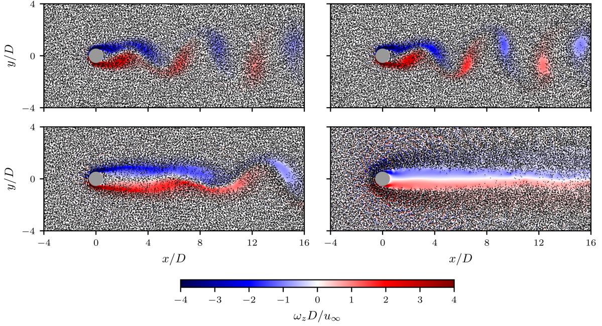
Figure 5.16 – Snapshot of particle positions and vorticity field at volume fraction \Theta = 20\% . Hydrogel ( \text{Stk} = 0.5 ): top/left; Glass ( \text{Stk} = 1 ): top/right; Iron ( \text{Stk} = 2.8 ): bottom/left; \rho^* = 100 ( \text{Stk} = 33.5 ): bottom/right.
