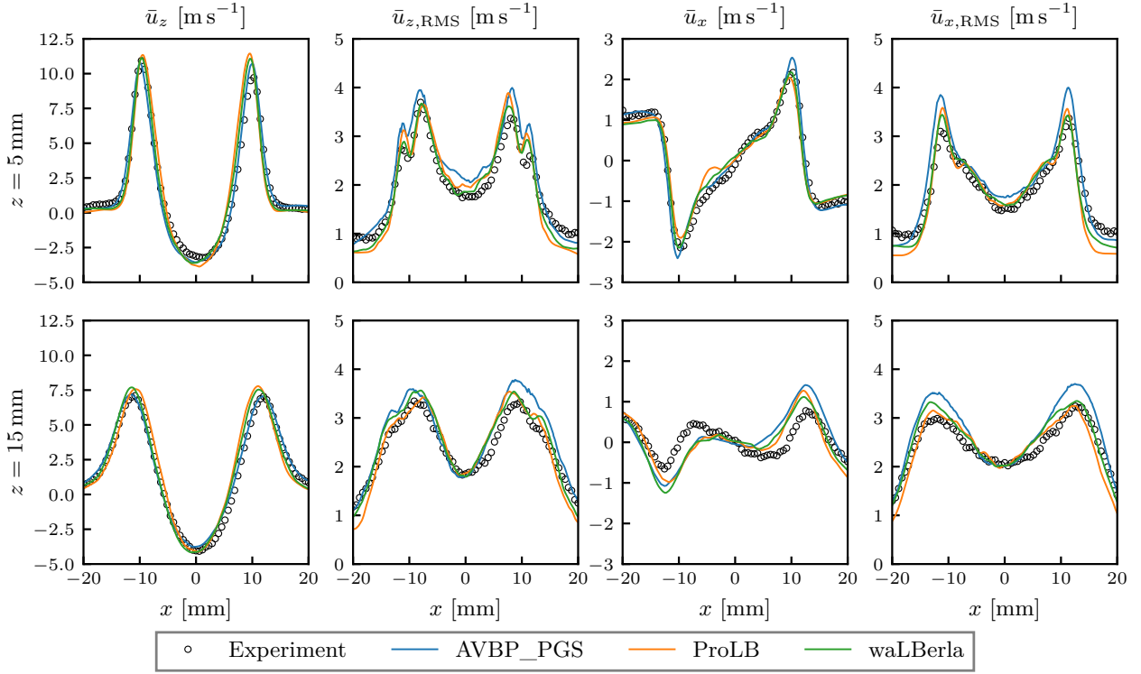
Figure 4.6 – Mean velocity profiles and related RMS of \bar{u}_z and \bar{u}_x for different solvers with. Obtained at constant axial coordinate on the axial plane. First and second rows correspond to z = 5 mm and z = 15 mm, respectively.
