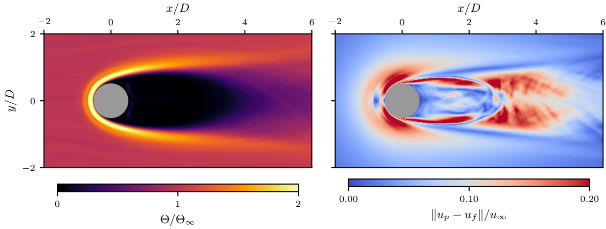
Figure 5.12 – Time averaged flow field of solid volume fraction and slip velocity of a suspension with iron particles, \Theta_\infty = 0.1 and \text{Re}_{\text{eff}} = 191 .
