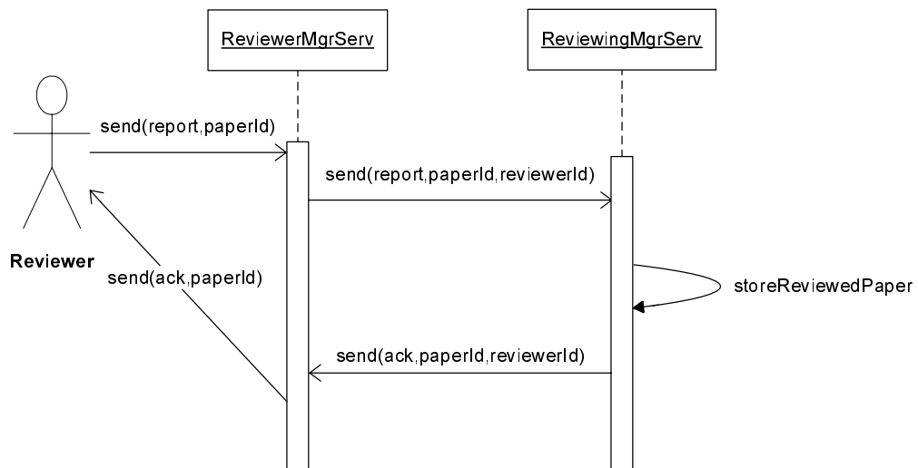
FIG. 5.6 – Transmission de rapports.
