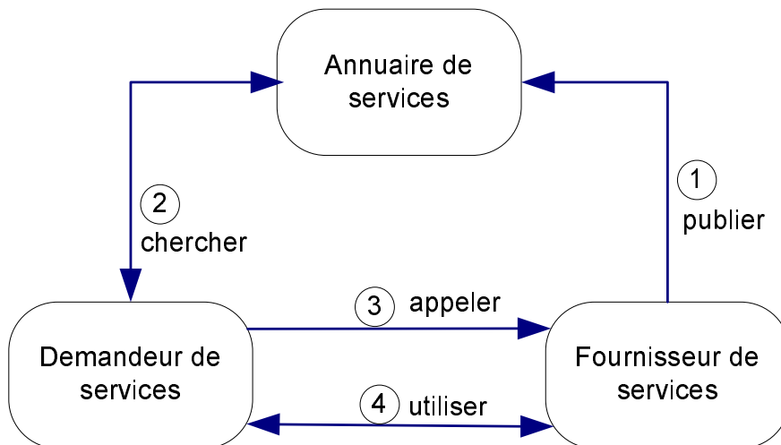
FIG. 2.11 – Architecture orientée service.
