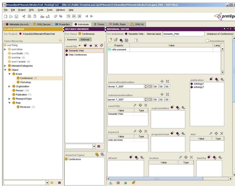
FIG. 6.7 – Instances de la classe Conference .
