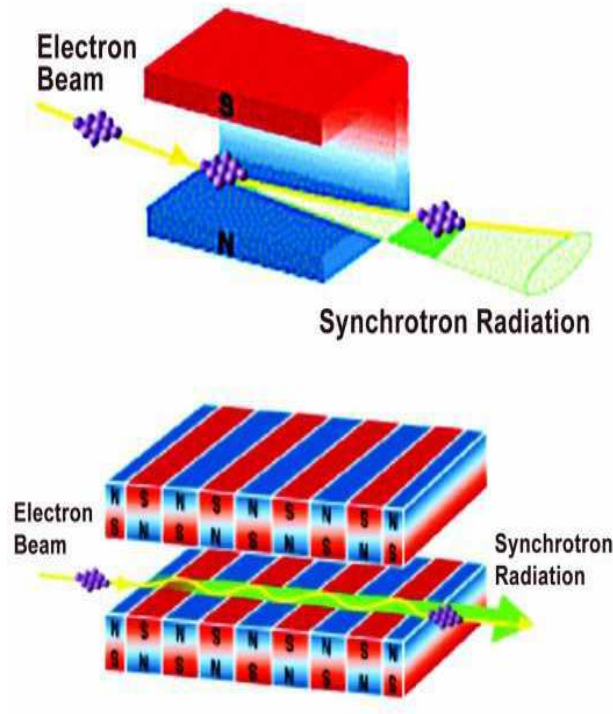
Figure 4.4: (Top) Schematic view of the generation of synchrotron radiation in a dipole bending magnet, where electron bunches are deviated to follow the orbit around the ring. (Bottom) Generation of synchrotron radiation in an insertion device, where the upper and lower magnet arrays produce vertical fields forcing the electrons to follow a zig-zag trajectory [109].
