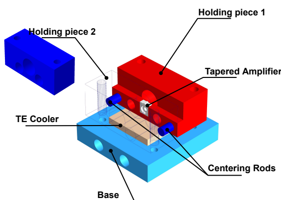
FIGURE IV.6 – Mechanical and thermal housing for the tapered amplifier (First-generation design)
