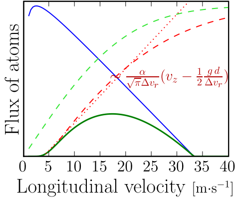
FIGURE V.9 – Effect of an acceleration The red dashed curve is the transfer function for the output tube of our setup, taking in account the deviation due to gravity. The blue curve is the 2D-MOT velocity distribution, the green dashed curve the transfer function with no deflection, and the thick green curved the output flux, taking into account the effect of gravity.
