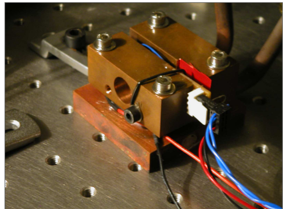
FIGURE IV.6 – Mechanical and thermal housing for the tapered amplifier (First-generation design)
