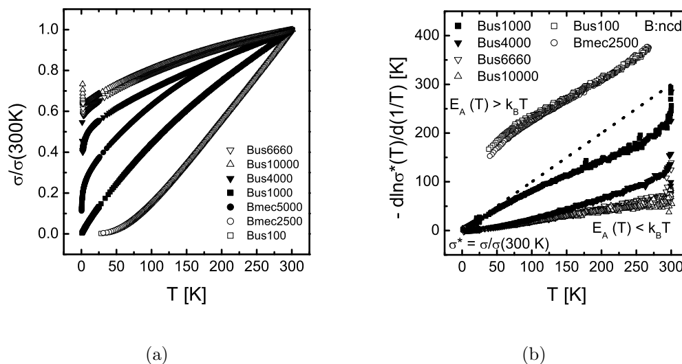
Figure 3.4.: (a) Temperature dependence of the normalized conductivity \sigma/\sigma(300K) for several samples in the range 300 K down to 350 mK. The highly doped sample with n_B = 3.3 \cdot 10^{21} \text{cm}^{-3} also shows superconductivity with a critical temperature T_c = 2.6K ; (b) Temperature dependence of the slope of the Arrhenius plots for the same samples. The Ioffe criterion as explained in detail in the text suggests a crossover from a thermally activated transport and, thus, insulating regime to a metallic regime. The critical concentration n_c for this crossover is estimated to be about 3 \times 10^{20} \text{cm}^{-3} as determined from SIMS.
