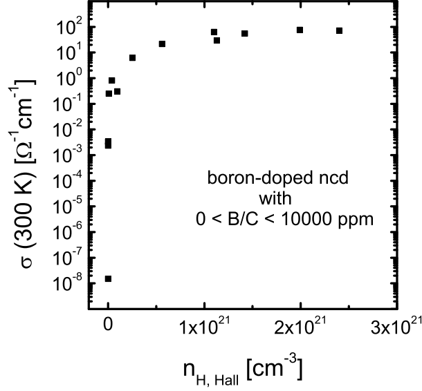
Figure 3.2.: Room temperature conductivity as a function of the free carrier concentration, as determined from room temperature Hall effect measurements, shown for several boron-doped nanocrystalline diamond thin films with boron concentrations (SIMS) in the range from 9.7 \cdot 10^{16} \text{ cm}^{-3} up to 3.0 \cdot 10^{21} \text{ cm}^{-3} (see Tab. 3.1). The strong increase of the conductivity with boron doping, from 10^{-8} (\Omega \text{cm})^{-1} up to 75 (\Omega \text{cm})^{-1} , already indicates the transition from the insulating to the metallic samples.
