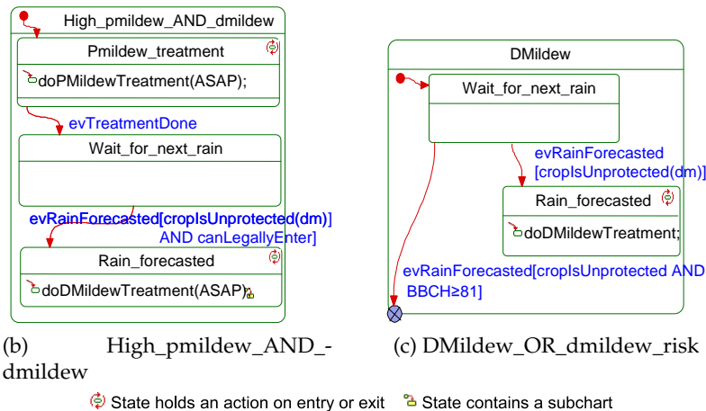
Figure 5.16: Substatecharts from Stage_5
