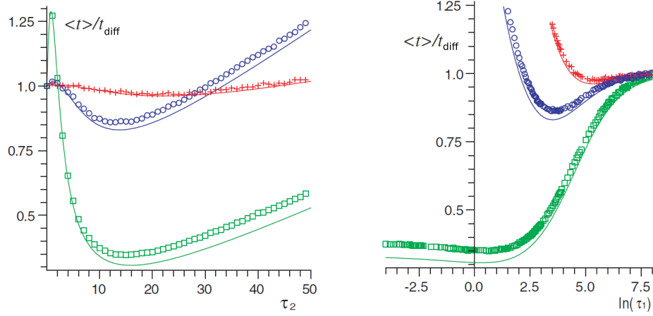
Figure 73: Diffusive mode in two dimensions. Simulations (symbols) versus analytical approximate (230) (line) of the search time, rescaled by the value in the absence of intermittence t_{\text{diff}} as a function of \tau_2 (left) and \ln(\tau_1) = (right), for D = 1 , V = 1 , b = 226 . Left : a = 10 , \tau_1 = 1.37 (green \square ); a = 1 , \tau_1 = 33.6 (blue \circ ); a = 0.1 , \tau_1 = 213 (red + ). Right : a = 10 , \tau_2 = 15.9 (green, \square ); a = 1 , \tau_2 = 13.7 (blue, \circ ); a = 0.1 , \tau_2 = 22 (red, + ).
