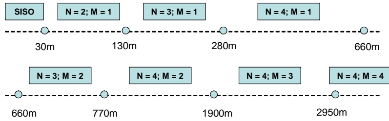
Figure 3.10: Optimal N - M transmit and receive antennas set selection as a function of transmission distance, FER = 10^{-3} requirement, Rayleigh block fading channel with power path-loss factor K = 2 .
