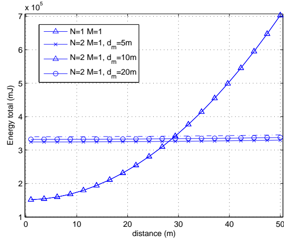
Figure 3.14: Energy consumption of the cooperative MISO 2–1 with different cooperative transmission distances d_m = 5, 10 and 20\text{m} , FER = 10^{-3} requirement, Rayleigh block fading channel with power path-loss factor K = 2 .
