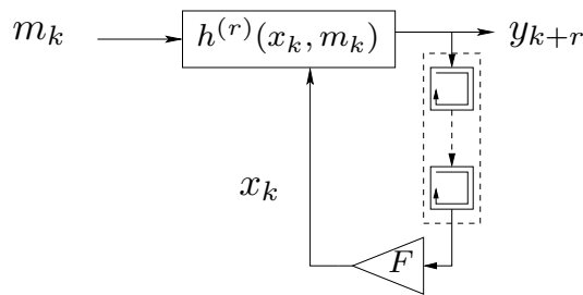
FIG. 4.1 – Self-synchronizing Message Embedded Stream Cipher
