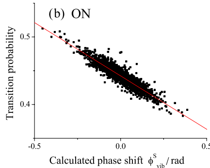
Figure 2. Correlation between the transition probability of the interferometer and the phase shift calculated from the seismometer data, for 2T = 100 ms. (a) The isolation platform is OFF. Grey points: without digital filter, black points: with digital filter. (b) The isolation platform is ON. Black points: with digital filter. Line: fit to the data, with correlation factor of 0.94.
