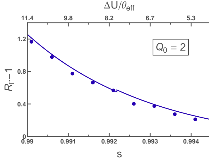
Fig. 3.12. Symbols: Rate asymmetry for Q_0 = 2 . \gamma_N=1.5 and \theta is fixed to have \theta_{\text{eff}} = 0.000165 . Solid lines: theoretical prediction (the slight jump in the line is due to a discontinuity between the two limits of Eq. (2.92)).
