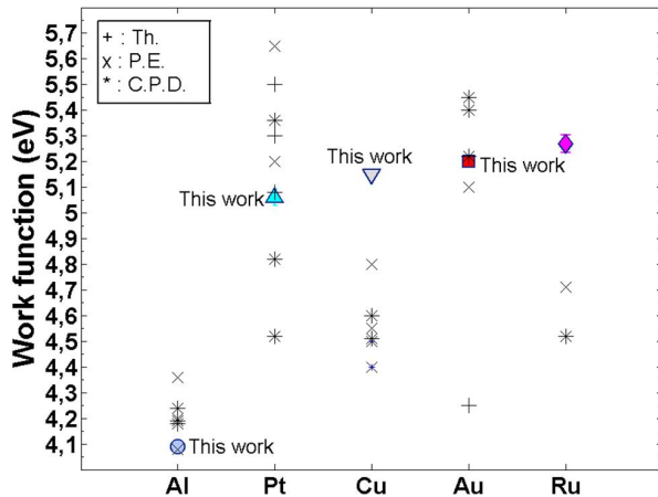
Figure 4.4: Work function values calculated from V_{cpd} obtained from the fit results in this work (colored motives). Results are compared to data reported from other studies as the work function has been measured by different techniques: Th. (thermoionic emission), P.E. (photo emission) and CPD (contact potential difference).
