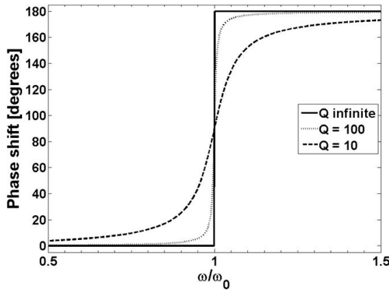
Figure 3.5: Phase shift behavior of a driven harmonic oscillator as a function of driving frequency. For ideal case ( Q = \infty ) there is a sharp transition from 0^\circ to 180^\circ at \omega_{ext} = \omega_0 . The damping produces continuous changes of the phase shift.
