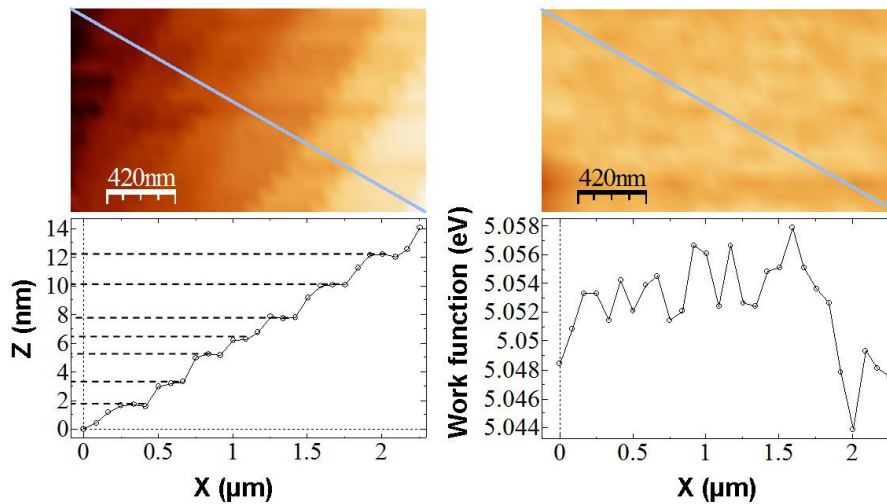
Figure 5.26: The topography (left) and work function (right) images magnified over the low work function values regions indicated by zone L in figure 5.22. Cross sections across the line drawn on the images clearly indicate a continuous increase of the topography following the terrace-like pattern of the SiC substrate.
