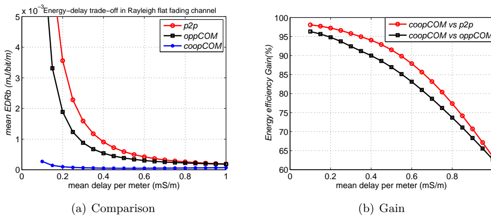
Figure 7.6: Energy gain of CMIMO in Rayleigh fading channel
