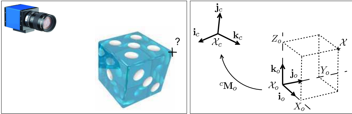
Figure 1.1: Representation of the 3D space using Euclidean geometry.
