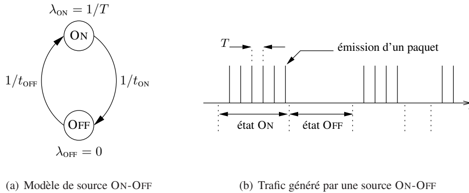
FIG. 4.4: Source ON-OFF
