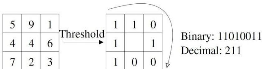
Figure 2.10: An example of the basic LBP operator [Ahonen et al. 2004].
