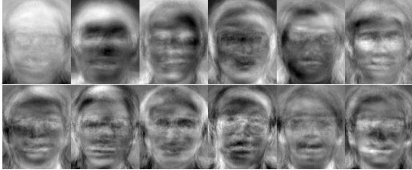
Figure 2.6: First 12 LDA basis vectors shown as resolution p \times q , where p \times q = n , derived from the ATT (ORL) face dataset.
