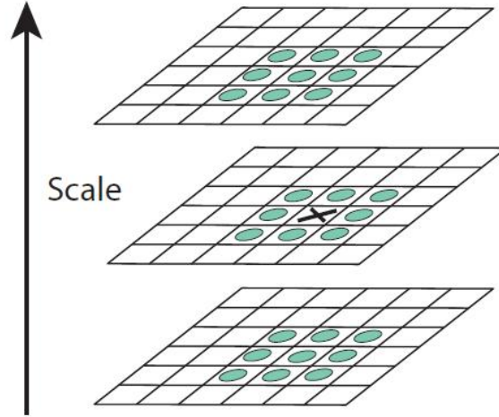
Figure 2.13: Maxima and minima of the difference-of-Gaussian images are detected by comparing a pixel (marked with '×') to its 26 neighbors in 3 \times 3 regions at the current and adjacent scales (marked with circles) [Lowe 2004].
