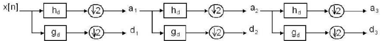
Figure 1.7: A three order Mallat decomposition tree.
