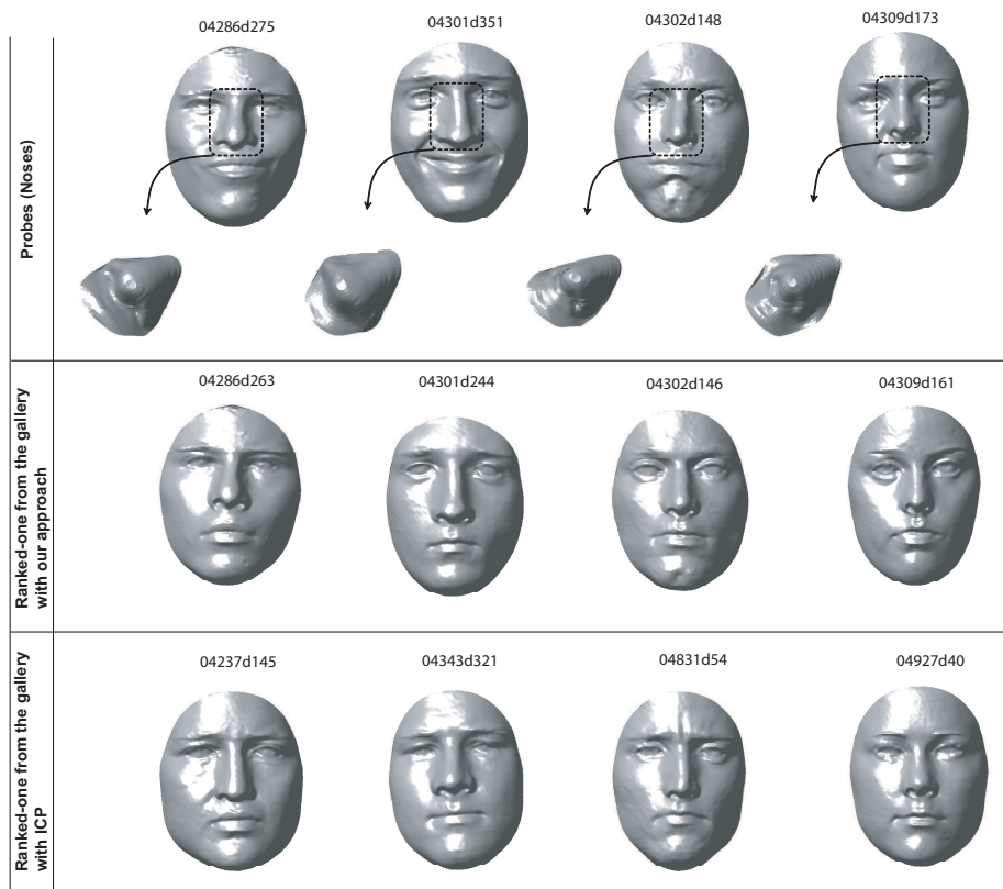
Figure 3.16: Examples of noses that are recognized by our approach and not by ICP algorithm on nose region
