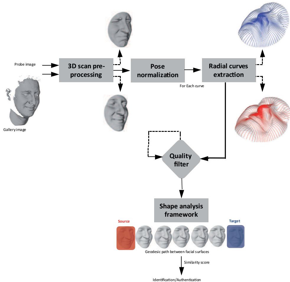
Figure 4.3: Overview of the proposed method.
