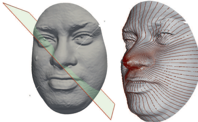
Figure 4.5: Radial curves extraction : left image illustrates the intersection between the face surface and a plan to form two radial curves. The collection of radial curves is illustrated at the right image.
