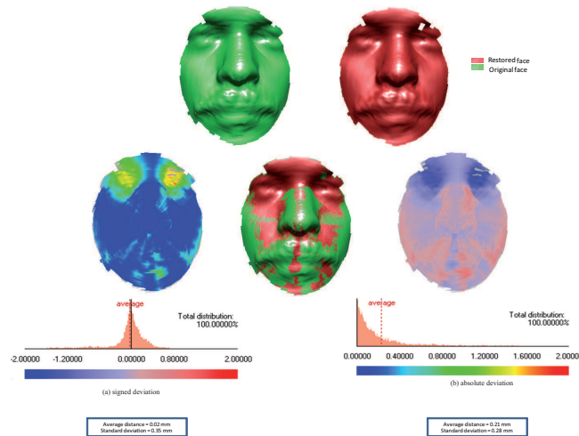
Figure 5.12: Restoration of full face. The absolute and signed deviations
