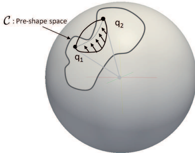
Figure 3.6: Illustration of the Pre-Shape Space \mathcal{C} and geodesic in this pre-shape space.
