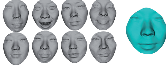
Figure 5.1: An example of Karcher mean of faces, the face at the right is the karcher mean of the eight faces in the left.
