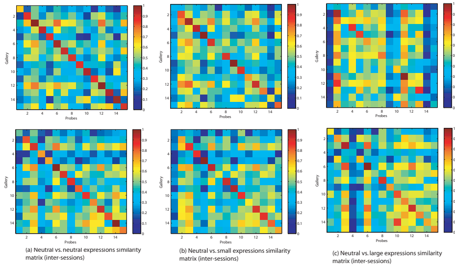
Figure 3.10: Similarity matrices for (a) neutral vs. neutral comparisons, (b) neutral vs. small expressions, and (c) neutral vs. large expressions, top row includes matrices for face-to-face matching and bottom row includes nose-to-nose matching.
