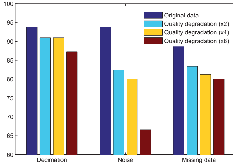
Figure 4.21: Recognition accuracy for different quality degradation experiments.
