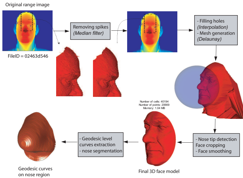
Figure 3.3: Automatic FRGC data preprocessing and nose curves extraction.
