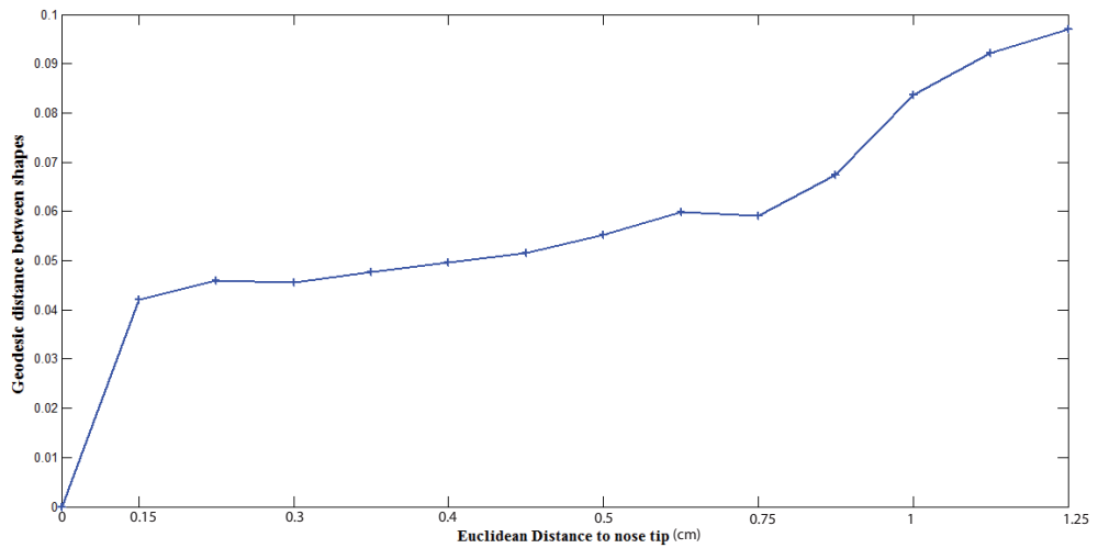
Figure 4.22: Variation in shapes of radial curves versus changes in locations of reference points.
