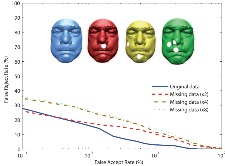
Figure 4.19: DET curves for experiments on missing data.
