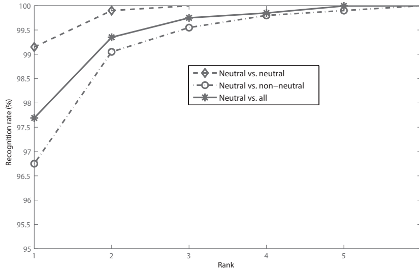
Figure 4.16: CMC curves of our approach for the following scenario: neutral vs. neutral, neutral vs. expressions and neutral vs. all.
