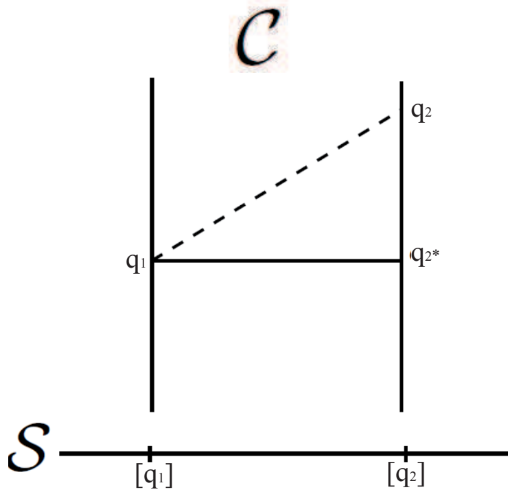
Figure 3.8: Computing geodesics in the quotient space.
