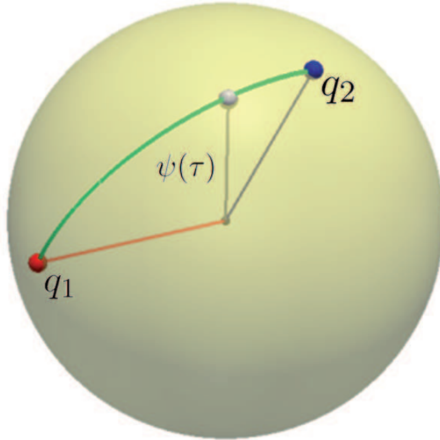
Figure 4.8: Illustration of shape space and geodesic between its elements.
