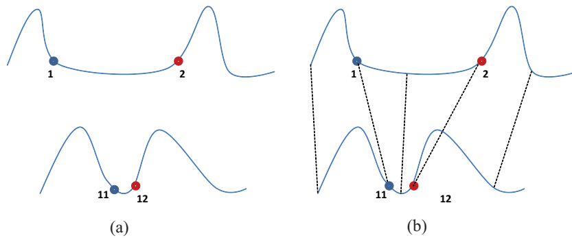
Figure 4.6: Illustration of elastic metric. In order to compare the two curves in (a), some combination of stretching and bending are needed. The elastic metric measures the amounts of these deformations. The optimal matching between the two curves is illustrated in (b).
