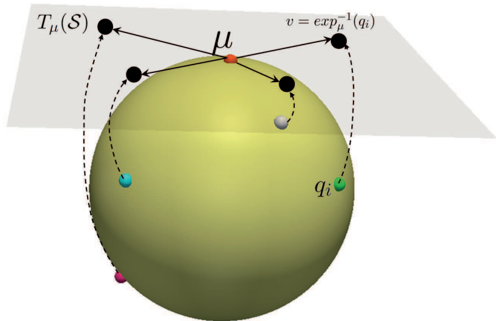
Figure 5.10: Illustration of mapping shapes onto the tangent space of \mu , T_\mu(\mathcal{S}) . Dashed arcs illustrate the projection of elements of the manifold to the tangent space.
