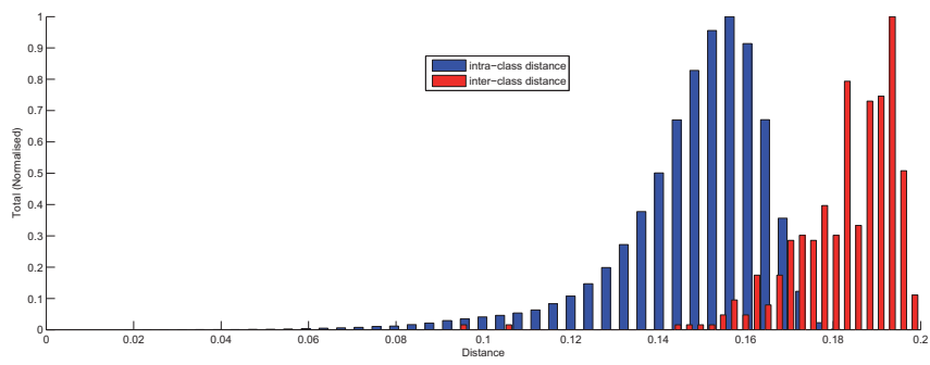
Figure 4.23: Distributions of intra-class and inter-class distances.
