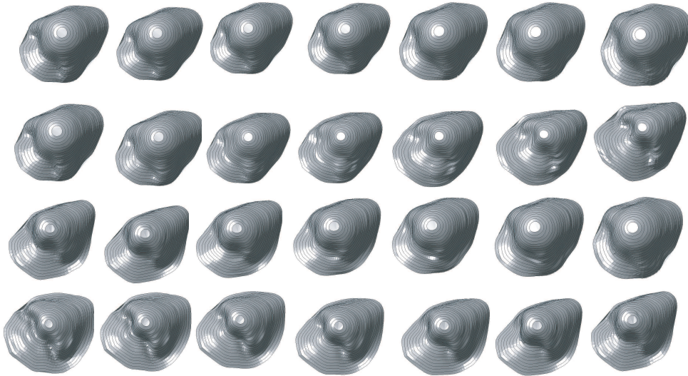
Figure 3.9: Geodesic path between source and target noses (a) First row: intra-class path, source and target with different expressions (b) Three last rows: inter-class path
