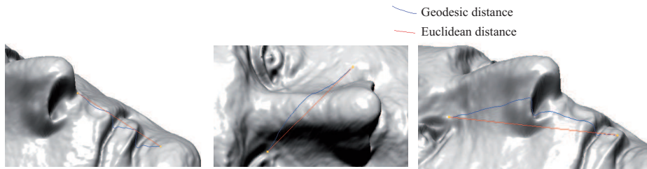
Figure 2.7: Euclidean path (in red) and geodesic one (in blue) on facial surface
