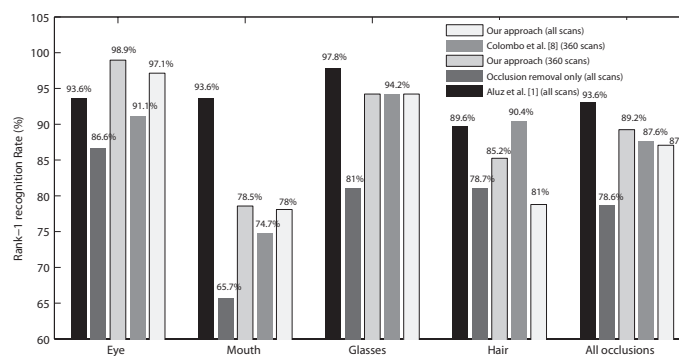
Figure 5.19: Recognition results on Bosphorus database and comparison with state-of-the-art approaches.
