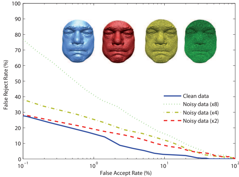
Figure 4.20: DET curves for experiments on noisy data.
