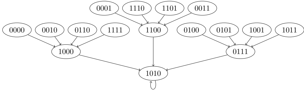
(a) f_{00}
