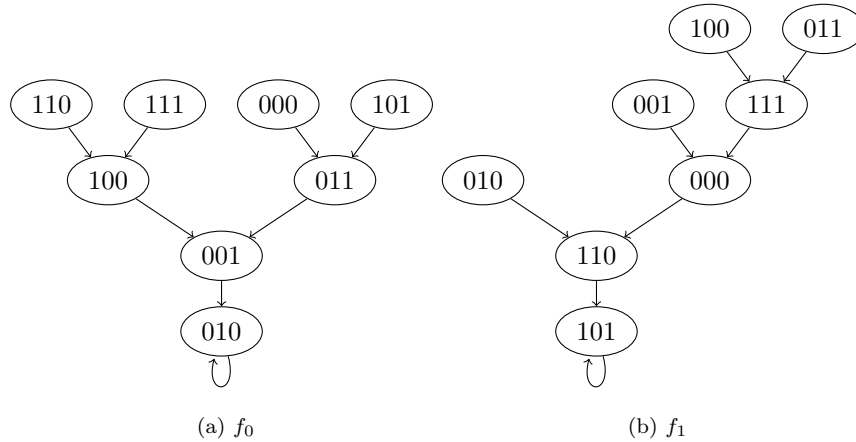
Figure 5.3: Graph of the functions f_0 and f_1
