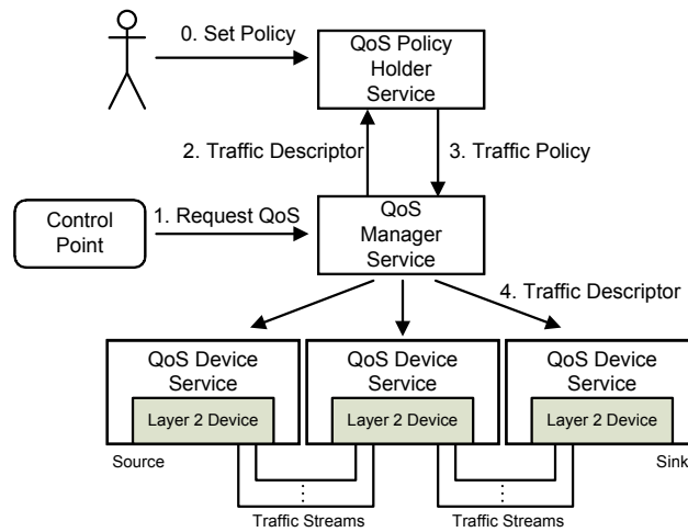
Figure 2.3: The UPnP QoS architecture (V3.0)
