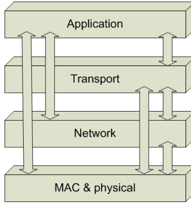
Figure 6.1: Interaction between adjacent and non adjacent layers
