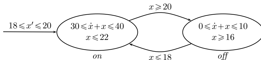
Figure 10.3: Hybrid automaton: Thermostat example (cf. [ACH + 95])
