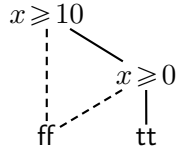
Figure 7.2: In this mixed BDD, the decision x \geq 0 is redundant (w.r.t. tt branch) and contradictory (w.r.t. ff branch).
