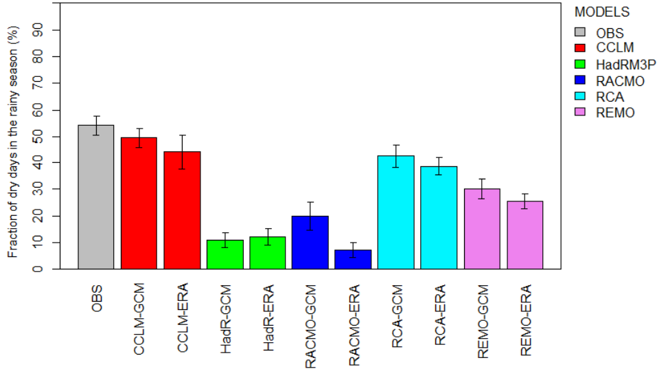
Figure 5.17: Average fraction of dry days in the rainy season in Burkina Faso from 1990 to 2004
