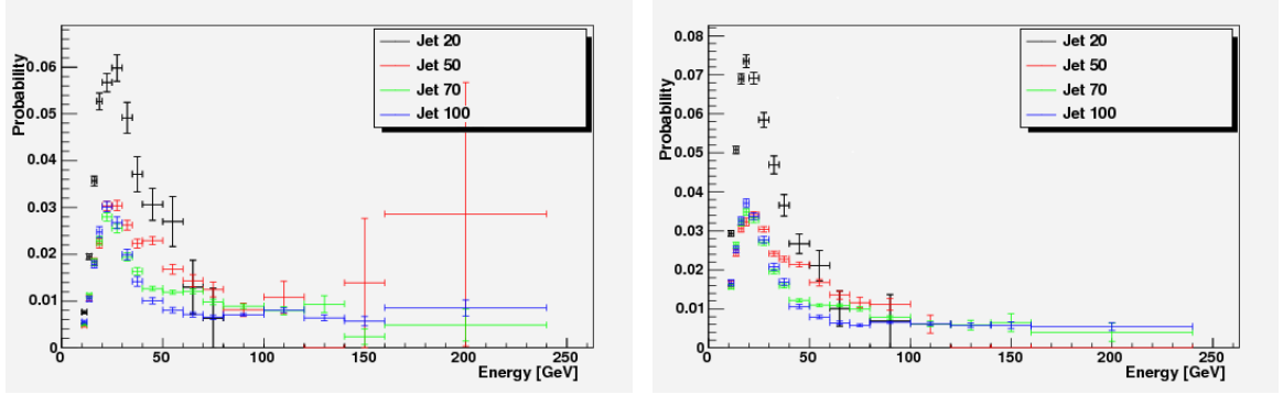
Figure 5.1: The \tau fake rate for periods from 18 to 28. On the left, the result for 1 prong taus, and on the right, 3 prong taus.
