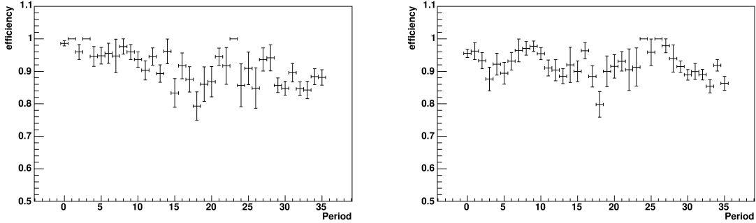
Figure 4.5: Trigger efficiency of one prong taus (left) and three prong taus (right), measured with the calibration CMUP muon sample, as a function of the run periods from very beginning of Run II until the end.
