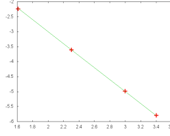
Figure 6.3: Log-log graph of N \mapsto \text{err}_N for N = 5, 10, 20, 30 . In green is the comparison with a line of slope -2 .
