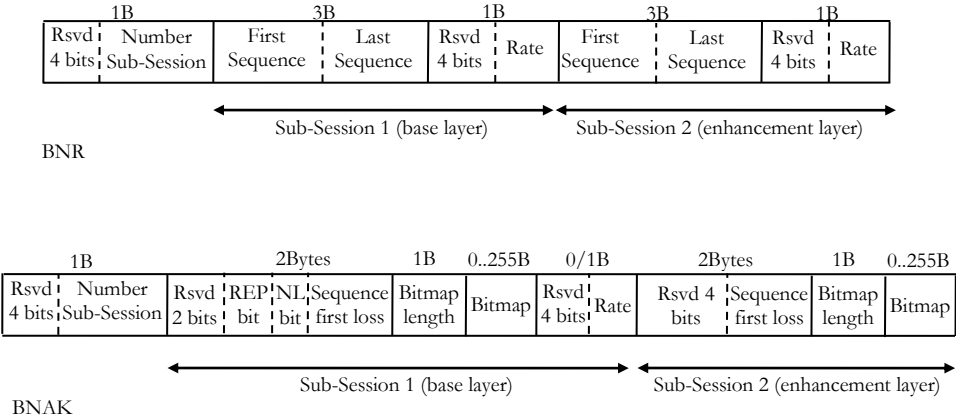
Figure 74. Packet format with one base layer and one enhancement layer
