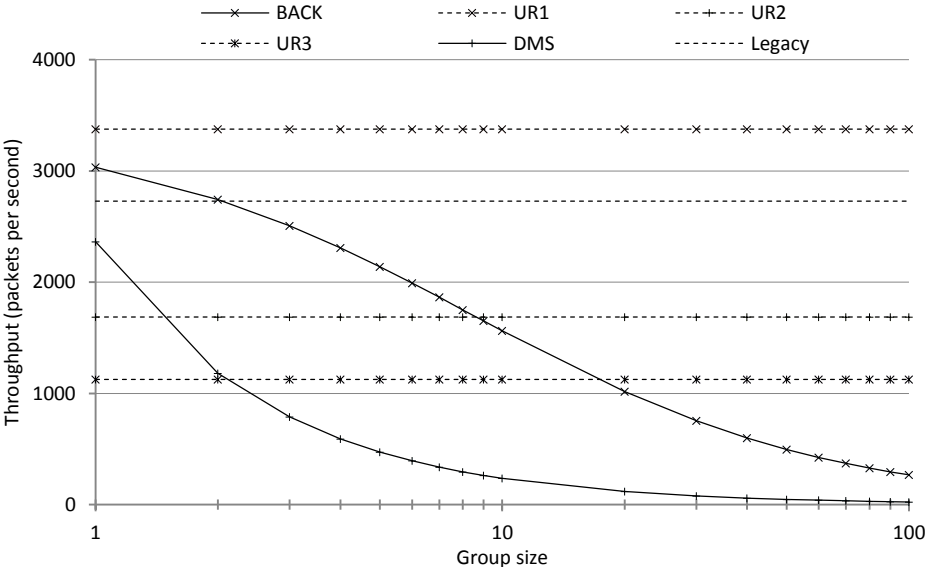
Figure 17. Throughput vs. group size
