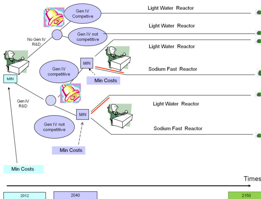
Figure 25: Decision tree
