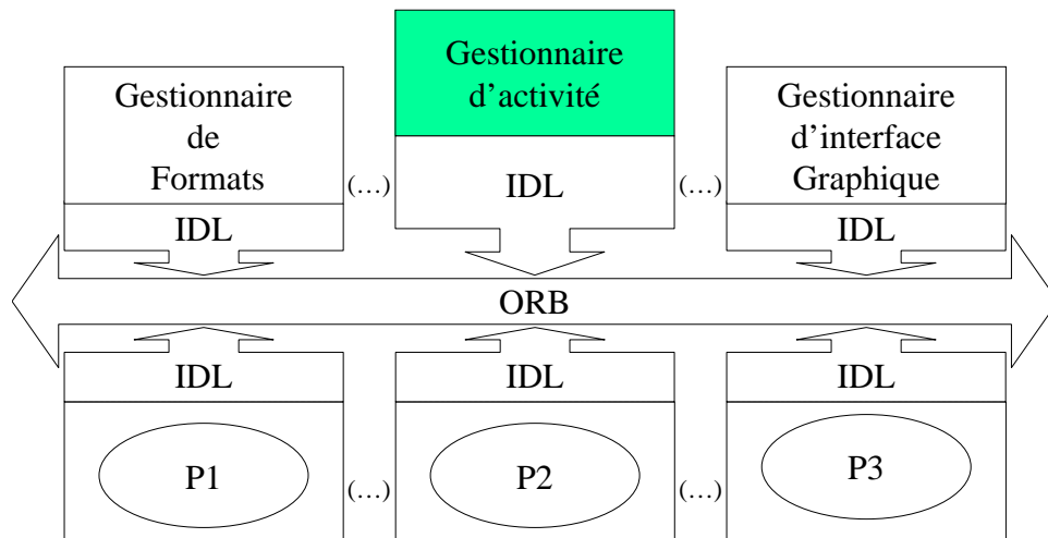
Figure 3.5 – Architecture d'EduMed
