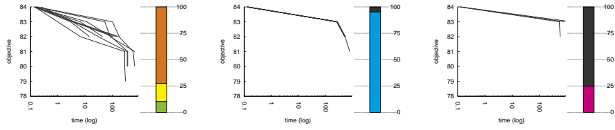
1.81 rcpsp_11 with PGLNS with 1.82 rcpsp_11 with cftLNS with 1.83 rcpsp_11 with ob-jLNS
