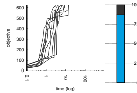
1.127 mario_mario_easy_2 with cftLNS
