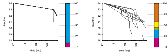
1.84 rcpsp_11 with EBLNS with 1.85 rcpsp_11 with PaE-GLNS
