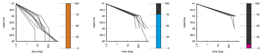
1.86 rcpsp_12 with PGLNS with 1.87 rcpsp_12 with cftLNS with 1.88 rcpsp_12 with ob-jLNS
