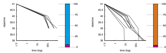
1.89 rcpsp_12 with EBLNS with 1.90 rcpsp_12 with PaE-GLNS
