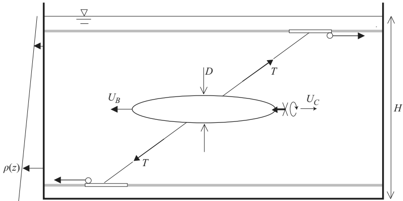
FIGURE 1. Experimental set-up.
