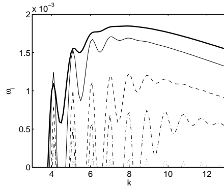
FIGURE 14. Maximum growth rate versus k of the second helical mode for Re = \infty . F = 2.5 (thick solid line), F = 3 (solid), F = 4 (dash), F = 5 (dash-dot), F = 7 (dotted)
