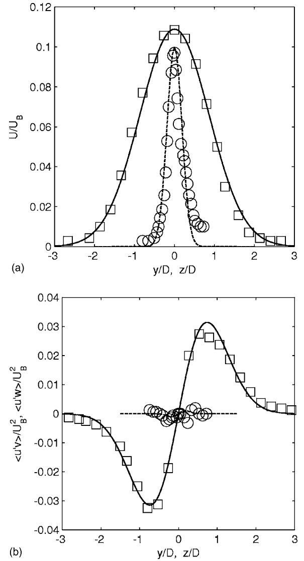
FIG. 2. Profile of (a) the mean velocity U and (b) the Reynolds stresses \langle u'v' \rangle and \langle u'w' \rangle for a sphere wake at Nt=20 for F=4 and Re=5 \times 10^3 . The data come from experimental results by Ref. 17 in the horizontal ( \square ) and vertical centerplane ( \circ ). The solid lines show a Gaussian profile for the mean velocity and the derivative of a Gaussian profile for the Reynolds stresses.
