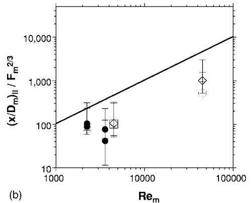
FIG. 8. Downstream distance x_{II} of the second transition, between a buoyancy-controlled (BC) regime and a quasi-2D regime (Q2D), as a function of (a) the Froude number and (b) the Reynolds number. Caption as in Fig. 7. The solid line corresponds to Eq. (21).
