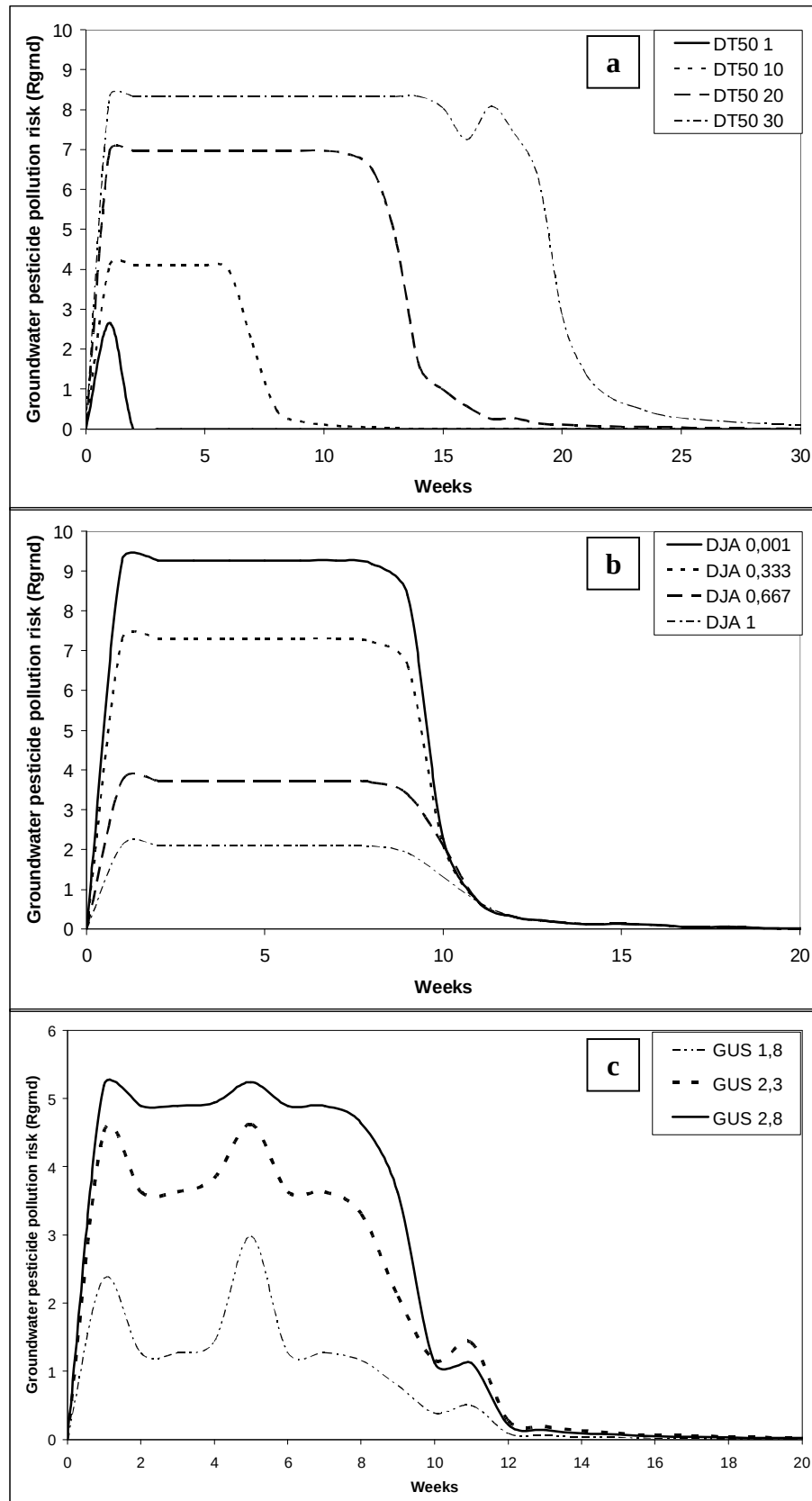
Fig. 8. Analysis of the sensitivity of the pesticide groundwater pollution risk indicator (Rgrnd)—under initial monoculture conditions with a pesticide treatment 5 weeks after planting—to variations in: a) the halflife DT50; (with ADI set at 0.5 and GUS set at 2); b) ADI (with Aquatox set at 0, DT50 set at 15 and GUS set at 2); and c) GUS (with ADI set at 0.5 and DT50 set at 15).
