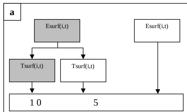
Flowchart for the pesticide pollution risk for surface water R_{surf}(i,t) .
