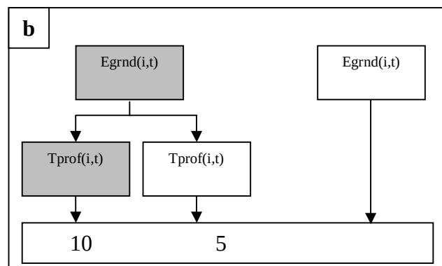
Flowchart for the pesticide pollution risk for groundwater R_{grnd}(i,t) .
