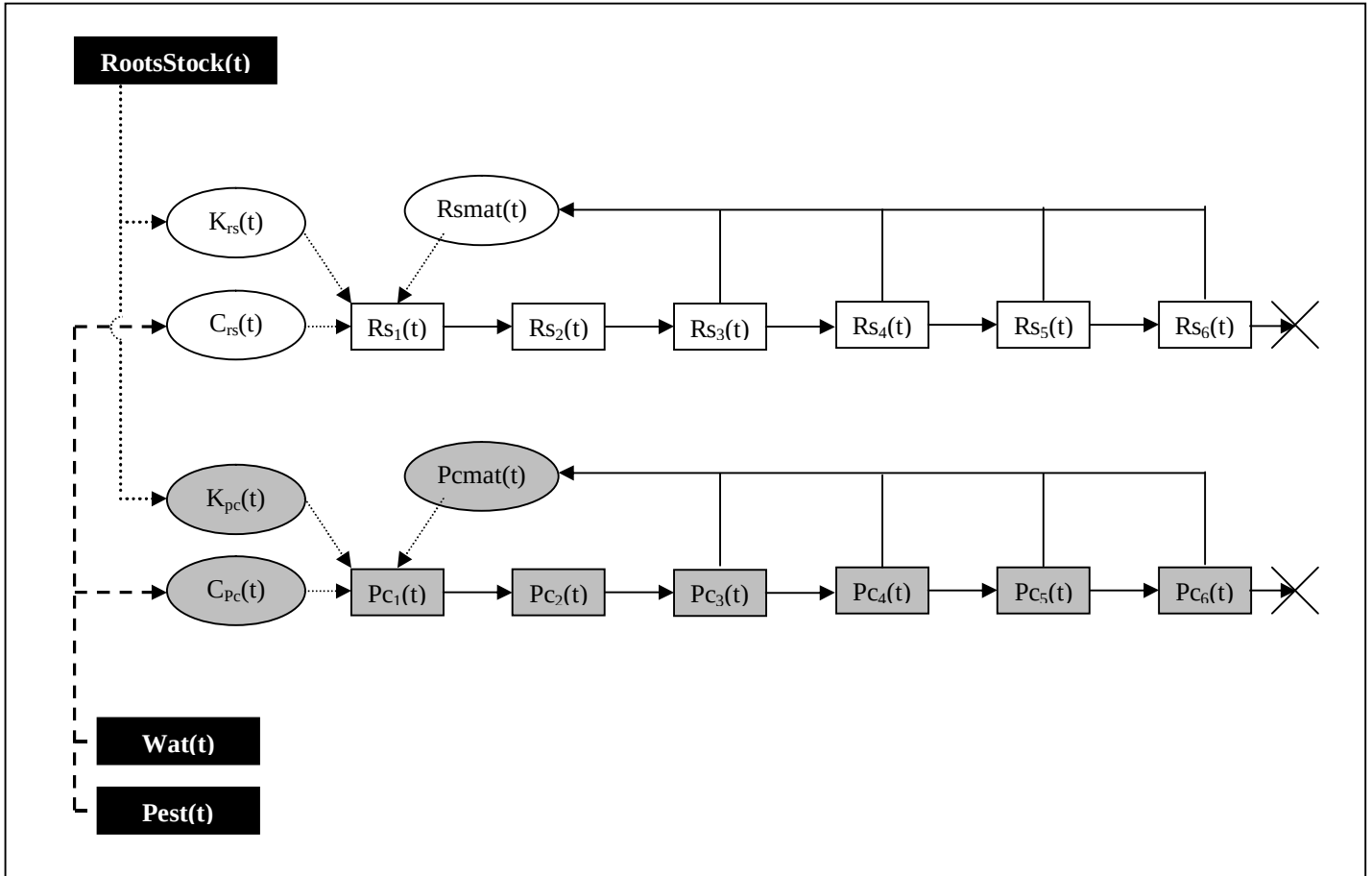
Fig. 1. Structure of the SIMBA-NEM model. With at each time step 't' of the model for each species, Rs(i)(t) and Pc(i)(t) representing the nematode number in the 'i' cohort, Rsmat(t) and Pcmat(t) the number of mature nematodes, Krs(t) and Kpc(t) the carrying capacity, crs(t) and cpc(t) the population growth parameter and RootsStock(t) , Wat(t) and Pest(t) the banana fresh root biomass, percentage of soil water and soil nematicide quantity, respectively.
