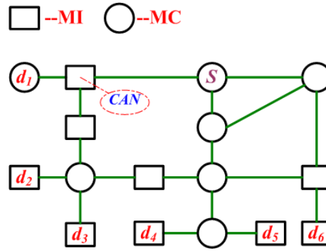
Figure 2.6: An Example Network with CAN Nodes
