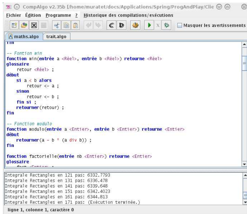
FIGURE 3.6 – Compalgo
