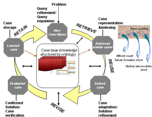
Figure 3.2. CBIR-CBR strategy
