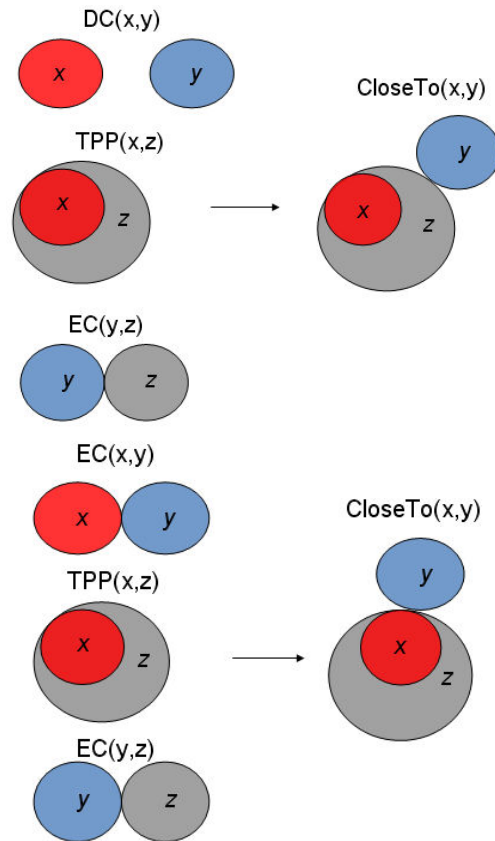
Figure 5.4. CloseTo relation
