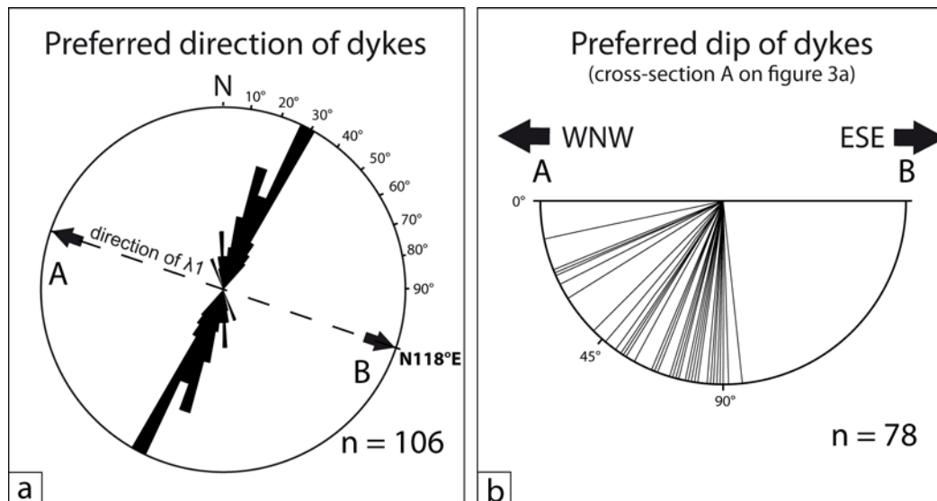
Figure 3. Results of the dyke array study. (a) Trend of the dykes plotted in lower hemisphere (equal area projection) highlighting a consistent N20°E -N30°E direction. (b) Apparent dip of the dykes projected along a stretching-parallel cross-section. n: number of measurements; because of their horizontal outcrop, dip of some dykes have not been determined.
