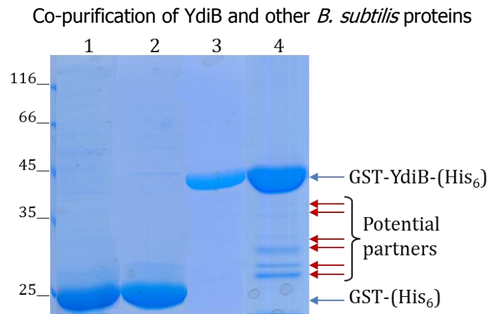
Figure S1: Co-purification of GST-YdiB-(His) 6 with other B. subtilis revealed by Pull-down method Purified GST-YdiB-(His) 6 and the control GST-(His) 6 , as the bait proteins, were incubated alone (lane 3 and 1 respectively) or with immobilized glutathione resin. Captured bait proteins were then incubated with B. subtilis lysate containing putative prey proteins. After washing to remove unbound proteins, retained components were eluted and separated by SDS-PAGE. Several additional bands were revealed in case of GST-YdiB-(His) 6 (lane 4) but not with the control GST-(His) 6 (lane 2). These bands containing potential partners of YdiB were then identified by mass spectrometry and presented in the (tab. x)
