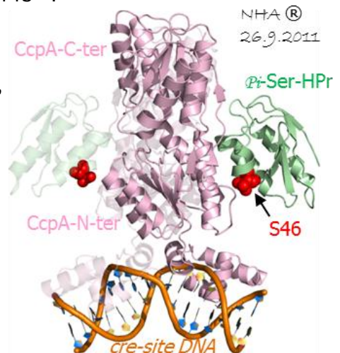
Figure 15 : CcpA/HPr/ ackA-cre structure complex 19
