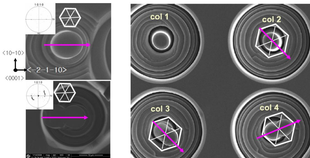
Figure 5.3: Massive shearing occurred along one of the three of \langle 11-20 \rangle directions. The apparent buckling or bending observed is not due to the misalignment of the flat punch tip or an inclination of the sample surface, since the direction of buckling is evenly distributed radially.
