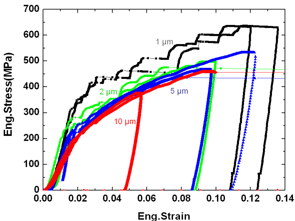
Figure 5.1: Size dependent stress-strain behavior of the [0001] orientation.
