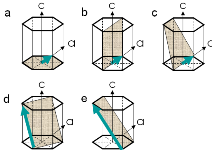
Figure 2.2: Deformation system of magnesium. (a), (b), (c) and (d) are basal, prismatic, pyramidal \pi_1 and pyramidal \pi_2 slip systems, respectively, whereas (e) is tensile twin system.
