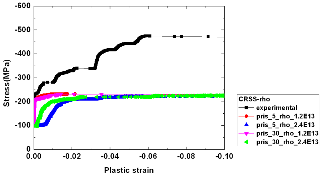
Figure 7.4 Stress-strain curves obtained for different CRSS of prismatic slip system and initial dislocation density. The CRSS values of basal, pyramidal \pi_1 and pyramidal \pi_2 slip system are 0.5, 100, 100MPa.
