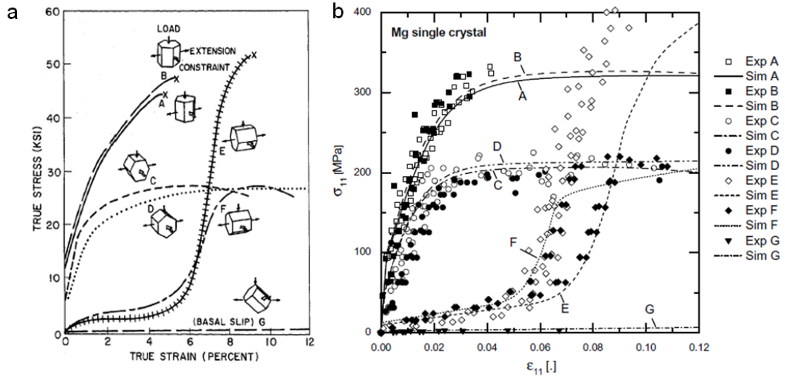
Figure 2.11 (a) experimental result of channel die test of Mg single crystal ([Kelly and Hosford 68]) (b) matched simulation result ([Graff et al. 07])
