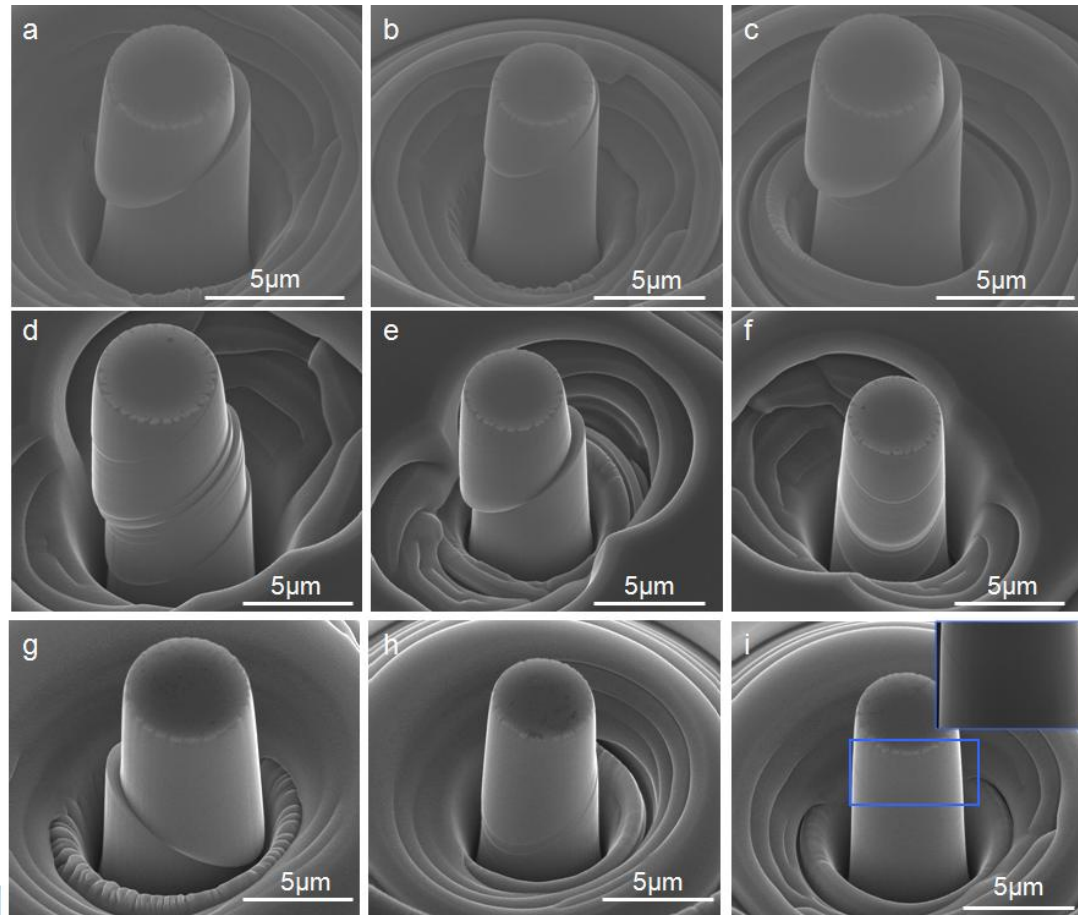
Figure 4.9: SEM micrographs of the post-compression microcolumns associated with the stress-strain curves given in Figure 4.8.
