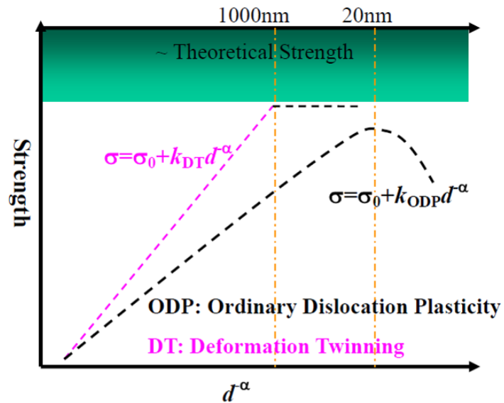
Figure 5.12: “Comparison of Hall-Petch scaling and Hall-Petch breakdown between ordinary dislocation plasticity (ODP, black curve) and deformation twinning (DT, magenta curve). Deformation twinning is much more size aware than ordinary dislocation plasticity in bcc and hcp metals.” ([Yu et al. 10])
