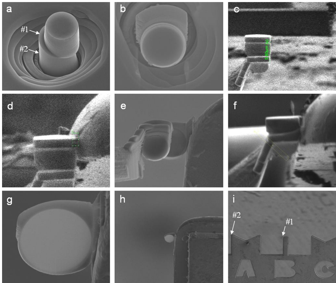
Figure 3.7: A novel method for TEM sample preparation of slip plane sections from compressed microcolumns. A section of the column where massive slip occurred is indicated by (#1) and a section parallel to #1 away from the massive slip is designated as (#2) and have been chosen for TEM foil preparation. Figure shows (a) initial (b) Pt deposition on slip plane (c) lift out, (d) mounting of bottom part #2 of column on copper grid, (e) cutting out of the middle part of column, (f) mounting of #1 on copper grid, (g) after thinning of #2, (h) after thinning of #1, and (i) an overview of copper grid with both TEM foils #1 and #2.
