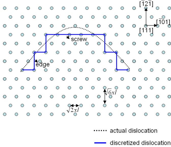
Figure 6.1: Edge-screw discretization of a dislocation line located in the (111) slip plane in TRIDIS code. The simulation lattice is defined by distance of ‘ xl ’. The out of plane direction is [111].
