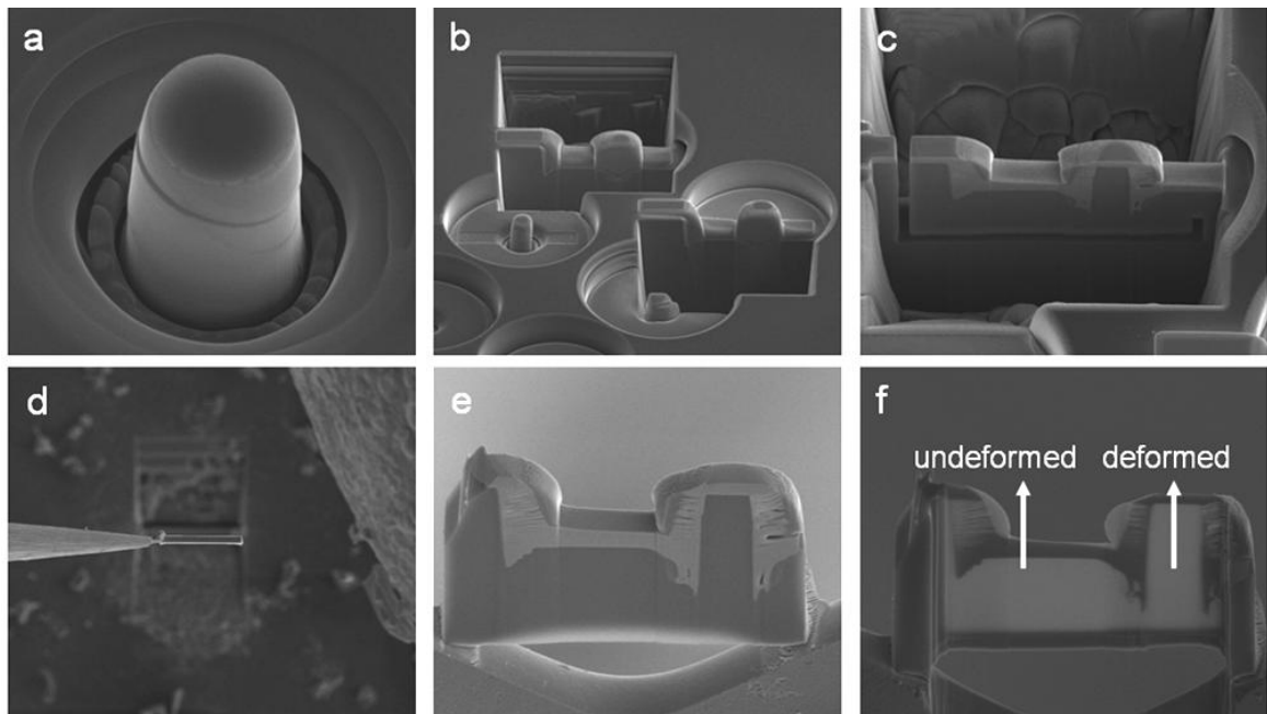
Figure 3.6: Typical working procedure of TEM sample by cross-sectioning. Figure shows (a) the initial deformed column, (b) regular and cleaning cross sections conducted on two columns, (c) through-cutting to partially free the lamella from the bulk material, (d) lift out of the lamella using an Omniprobe micromanipulator, (e) mounting of the lamella on a copper TEM grid, and (f) thinning to electron transparent thickness.
