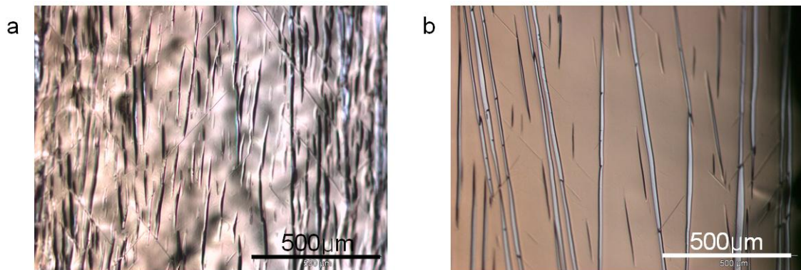
Figure 3.2: Optical micrographs of sample surface (a) after spark erosion and (b) after mechanical and electro polishing. The narrow needle-like structures are twins.
