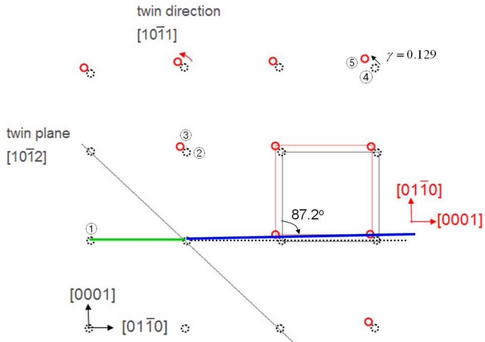
Figure 4.23: Formation of <c> component dislocation from transforming of the <a> type dislocation.
