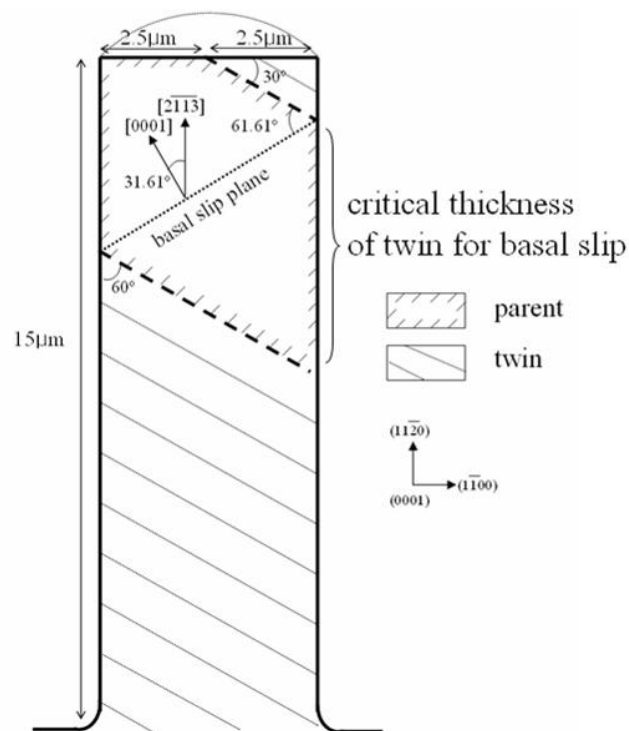
Figure 4.18: Schematic of a microcolumn used to compute the critical twin thickness needed to activate a basal slip band which extends across the entire column diameter.
