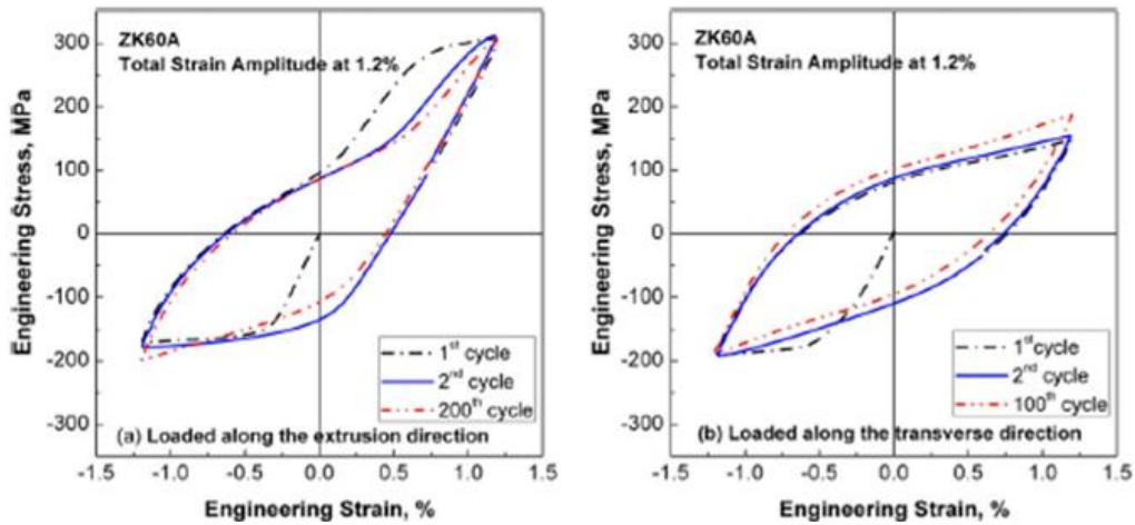
Figure 2.9: Strain hysteresis due to twinning during cyclic loading is shown with two loading direction ([Wu et al. 08]).
