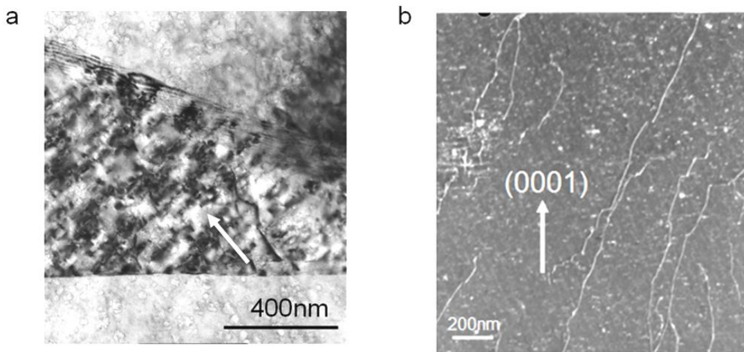
Figure 4.22: <c> component dislocations are observed in (a) a twin at the early stage of deformation, as well as in (b) the twinned region after the whole column is twinned.
