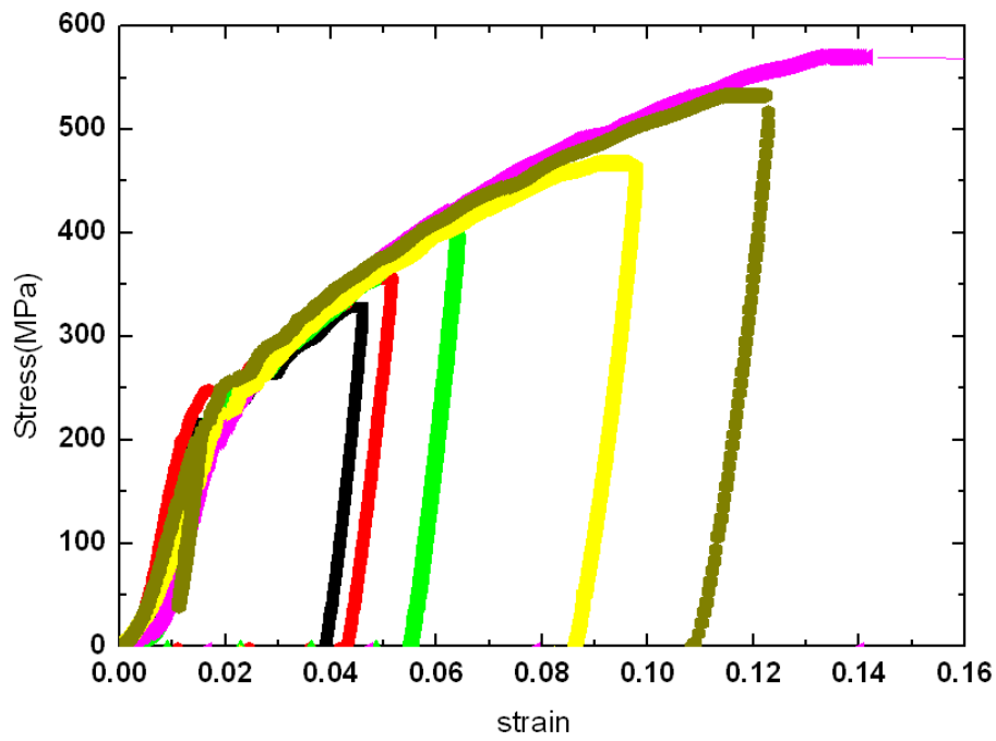
Figure 4.1: Stress-strain behavior of 6 microcolumns with nominal mid-height diameter of 5 \mu m.
