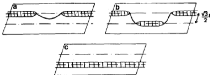
Figure 2.6: Kink-pair mechanism. ([Couret et al. 85]).
