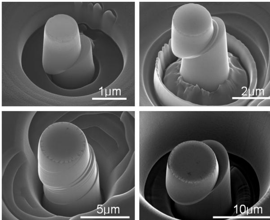
Figure 5.5: SEM images of deformed [2-1-12] pillars of varying size.
