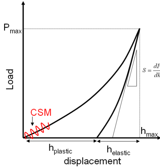
Figure 3.12: Schematic of the load-displacement trace achieved during nanoindentation testing.
