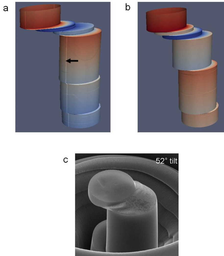
Figure 7.11: Deformed shape of the pillar compressed along [0001]. DD image processing was applied to (a) and (b). The CRSS of basal, prismatic, pyramidal \pi_1 and pyramidal \pi_2 is 0.5, 5 , 100, 100, respectively for the case of (a), whereas 0.5, 30 , 100, 100, respectively for the case of (b). The black arrow in (a) indicates a typical slip mark corresponding to prismatic slip. The actual deformed pillar is given in (c) for comparison.
