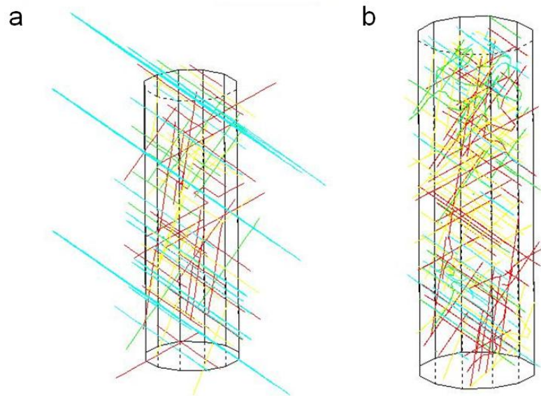
Figure 7.14: Tilted view of the simulated volume. (a) Total dislocation microstructure including bulk and virtual segments. (b) Bulk only dislocations contained in the pillars.
