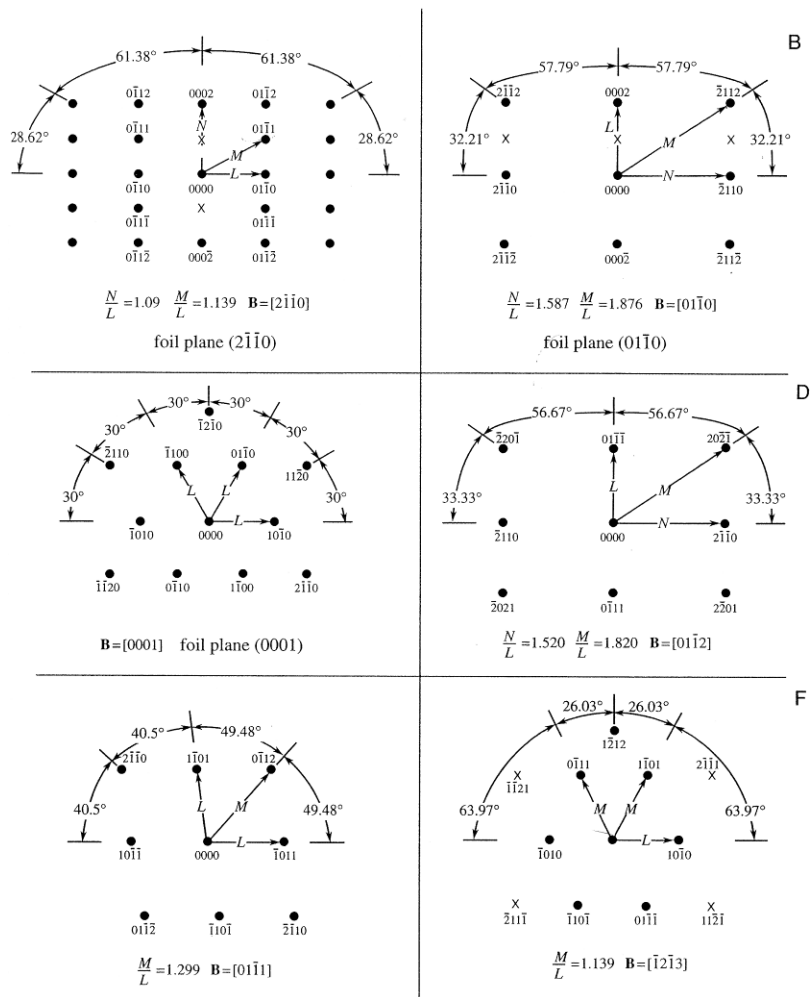
Figure 3.10: The principle diffraction patterns needed for investigating Mg, a hcp structure ([Williams and Carter 04]).
