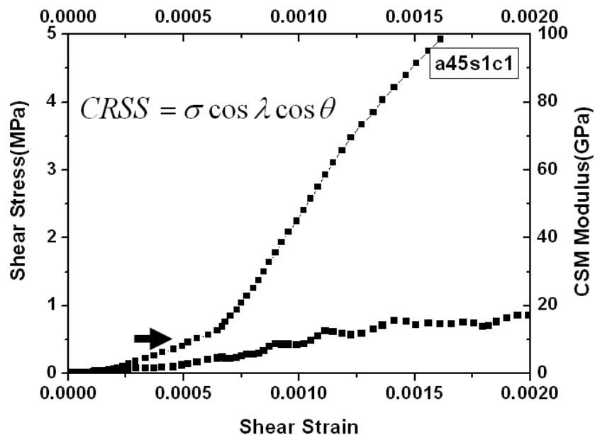
Figure 4.14: A plot of resolved shear stress (small squares) and CSM modulus (large squares) during the initial compression of a column oriented 45 degrees from the basal plane. An estimation of the CRSS of the basal slip system by identifying deviations in the slope of the stress-strain curve is complicated by the evolving contact inherent to compression testing.
