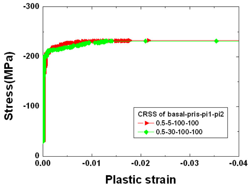
Figure 7.7: Typical DD simulation results for the [0001] orientation with two values for the CRSS on the prismatic system.
