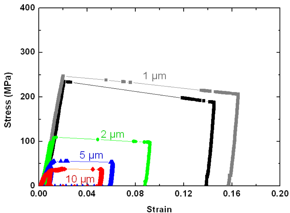
Figure 5.6: Stress-strain behavior of the [11-20] orientation pillars of varying size.
