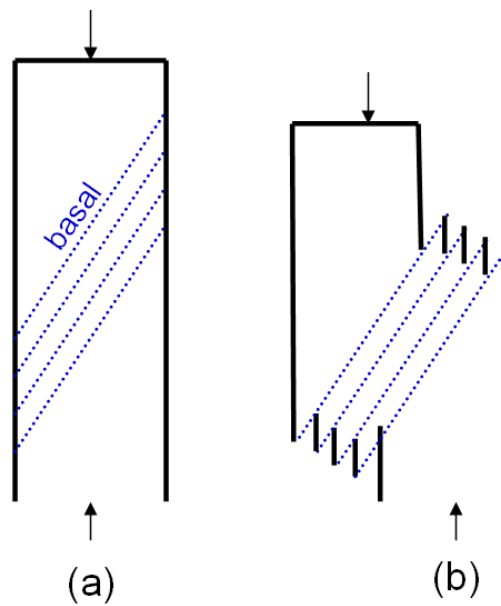
Figure 7.15: Schematic description of the deformation process in the case of [2-1-12] orientation. (a) initial (b) activation and glide of numerous basal dislocation.
