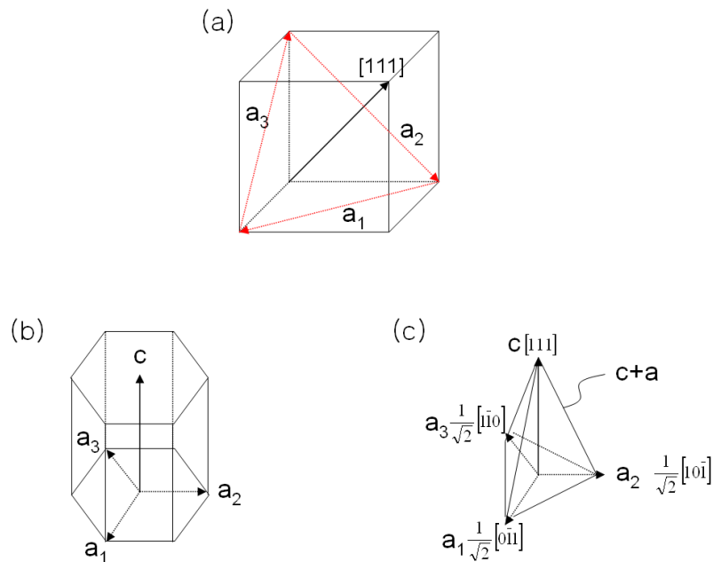
Figure 6.2: Conversion of TRIDIS-fcc to the hcp structure: (a) Burgers vectors in fcc structure (b) Burgers vectors in hcp structure (c) conversion of Burgers vectors
