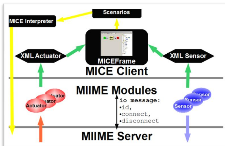
Figure 28 : Architecture ArCo
