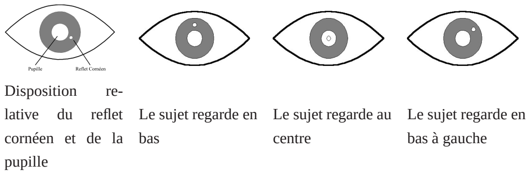
FIGURE 3.14 – Principe du reflet cornéen. Source [103].
