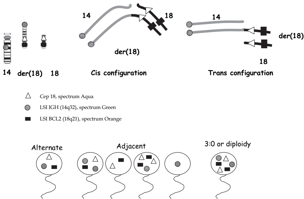
Figure 2. Ideogram of the chromosomes involved in the rearrangement and the probes used. The trivalent ( cis and trans configurations) and the various segregation patterns are schematized.
