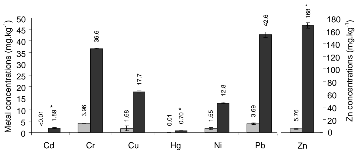
Fig. 2 (Figure 52) : Mean ( \pm SD) sediment metal concentrations ( \text{mg.kg}^{-1} dry weight) in the two caging stations ( \square A and \blacksquare B). * Concentration that exceeds the ERL (effects range-low) defined by Long et al. (1995).
