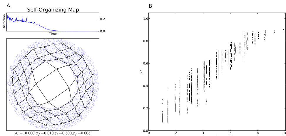
Figure 2.3: SOM on a uniform ring distribution. A Uniformly drawn input data on a ring. The white discs and the black grid represent the SOM neurons and the connections of them, respectively. The Distortion is computed during the simulation and it is depicted over time on the top of this panel. B The dx - dy representation of the present SOM.
