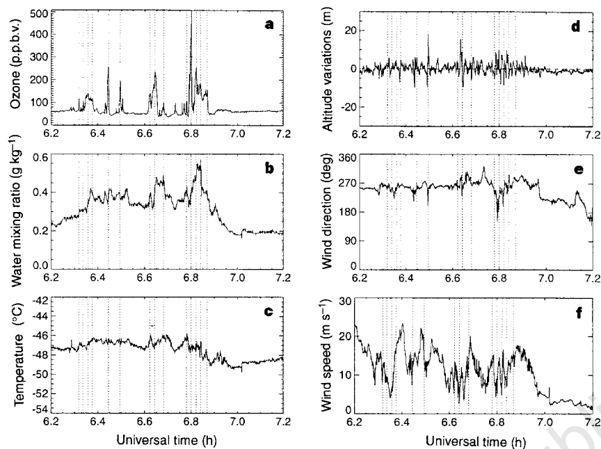
Figure 1 Time series of: a , ozone mixing ratio; b , water vapour mixing ratio; c , temperature; d , barometric flight altitude variations; e , wind direction; f , wind speed. These time series were measured on MOZAIC flight Paris-São Paulo on 21 November 1994. The time of the encounter of ozone maxima are marked by vertical dashed lines on all graphs. This time series represents one hour of measurements during which the aircraft travelled 860 km from 7° 20' N, 27° 20' W to 0° 30' N, 30° 20' W. (data acquisition every 4 s, resulting in a spatial resolution of about 1 km). Before and after the event shown here, ozone mixing ratios were always well below 100 p.p.b.v. in tropical latitudes. Instrumentation was as follows: a , a dual-beam ultraviolet absorption instrument, Thermo-Electron model 49-103 (detection limit 2 p.p.b.v., overall precision \pm 2\% ); b and c , an AERODATA AD-F8-88 instrument installed in a Rosemount housing; d , e , f , Airbus A340 on-board instruments. Documentation of ten representative cases is available on the ftp site ftpaero.aero.obs-mip.fr (file: /pub/salsa/mozaic/SUPP1.PS).
