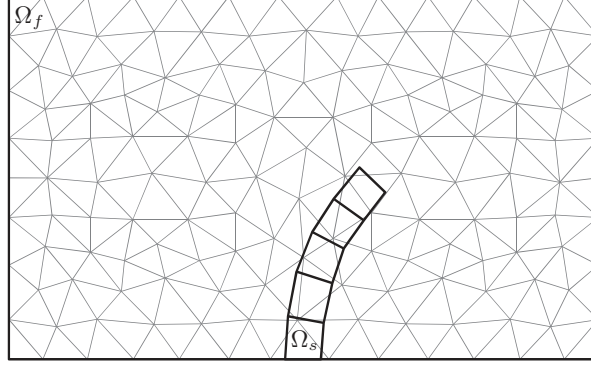
Figure 3.1: Schematic representation of the discretized problem in 2D.
