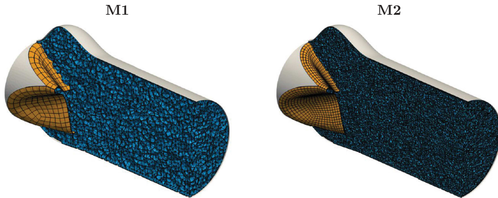
Figure 4.4: Computational zone of interest composed of the valve solid mesh and the aortic fluid mesh. Two levels of mesh are considered, the coarse mesh M_1 and the fine mesh M_2 .
