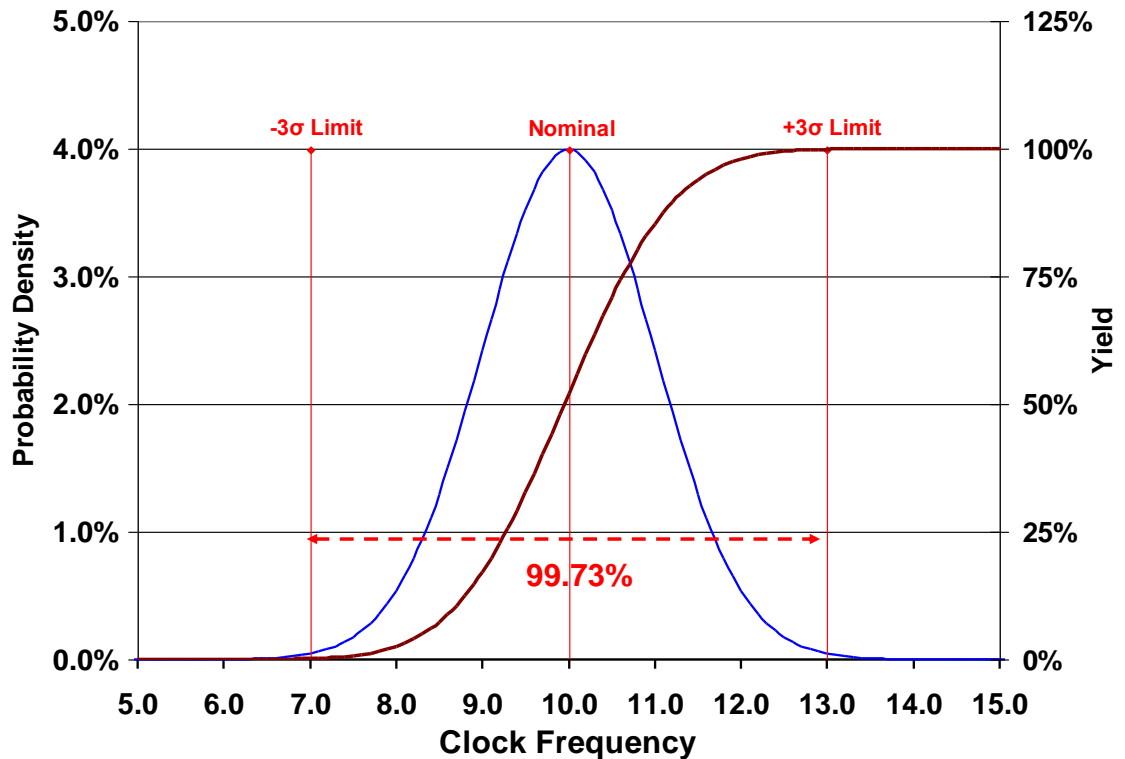
Figure 2-3: Yield histogram
