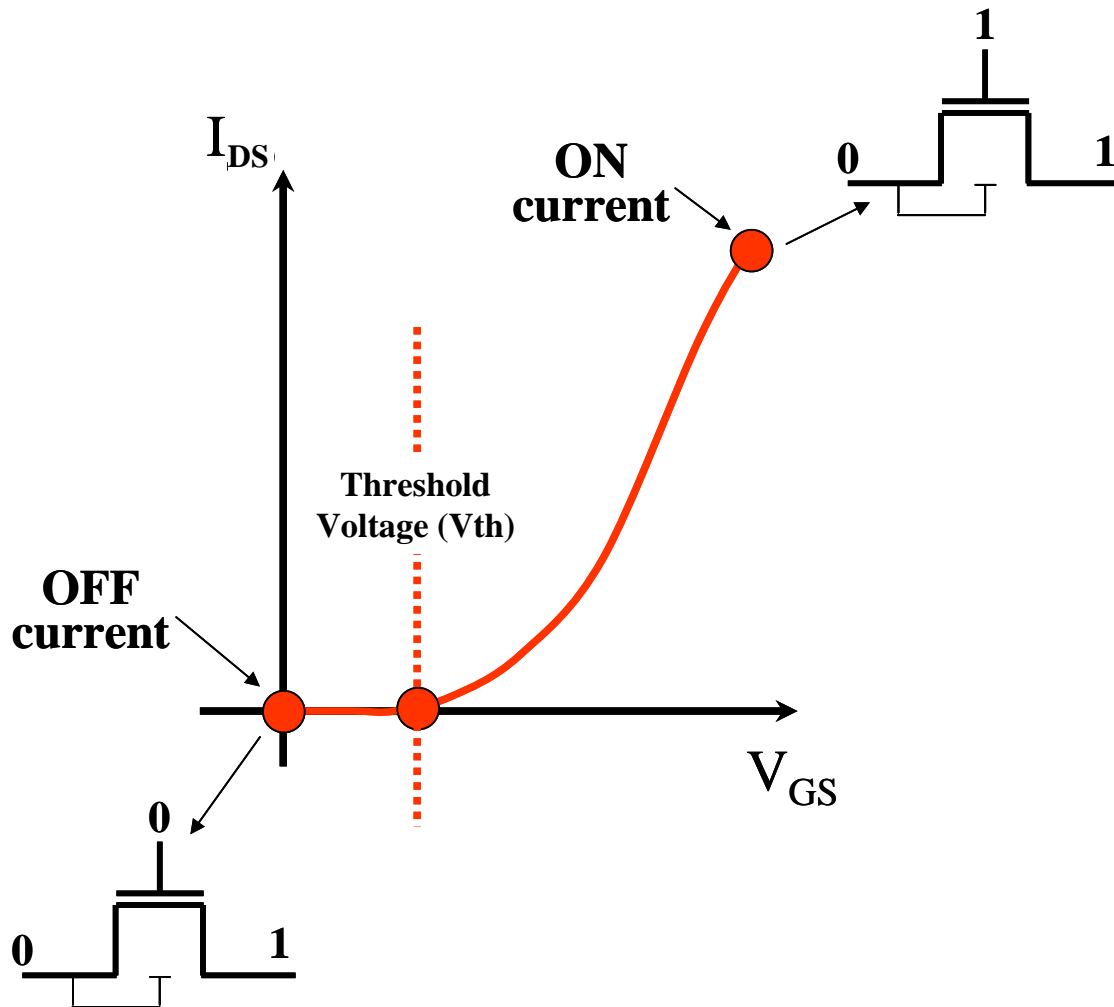
Figure 2-1: Drain current vs. gate voltage
