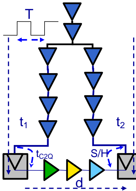
Figure 1-4: Impact of skew on setup/hold configurations
