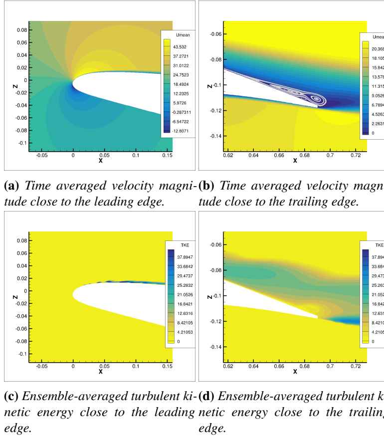
Figure 4.8: Contours of velocity and turbulent kinetic energy, 2D simulation with M1 grid for Re = 1M , angle of attack \alpha_o = 10^\circ . The detachment is shown by streamlines close to the trailing edge.
