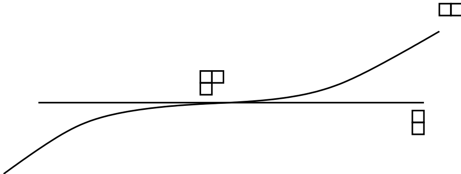
FIGURE 1. One of Kazarian's "generic" bifurcation diagrams. The curves intersect cubically at the origin (like the plane curves of equation y = x^3 and y = 0 at the origin). One of the components corresponds to the curves having a degenerate flattening point of anomaly sequence 2 while for the other component the anomaly sequence is (1, 1) .
