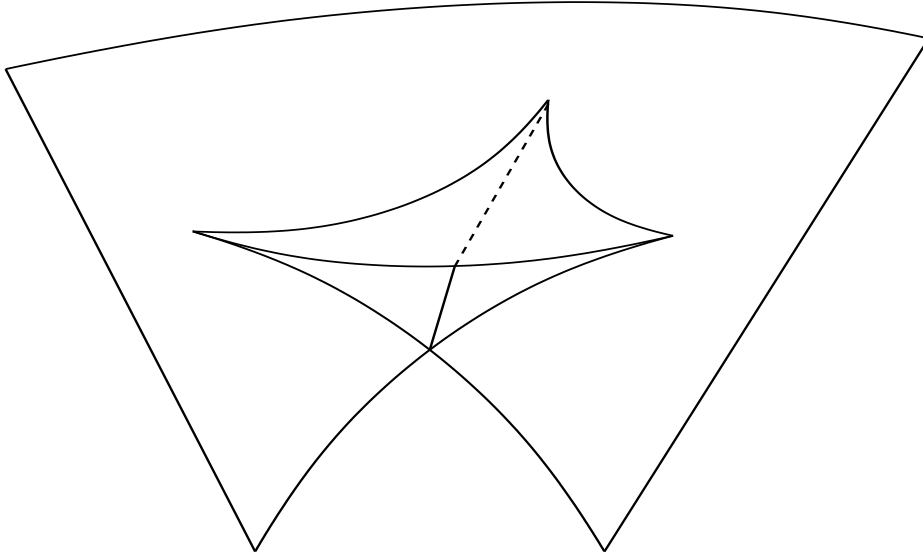
FIGURE 3. The swallowtail.
