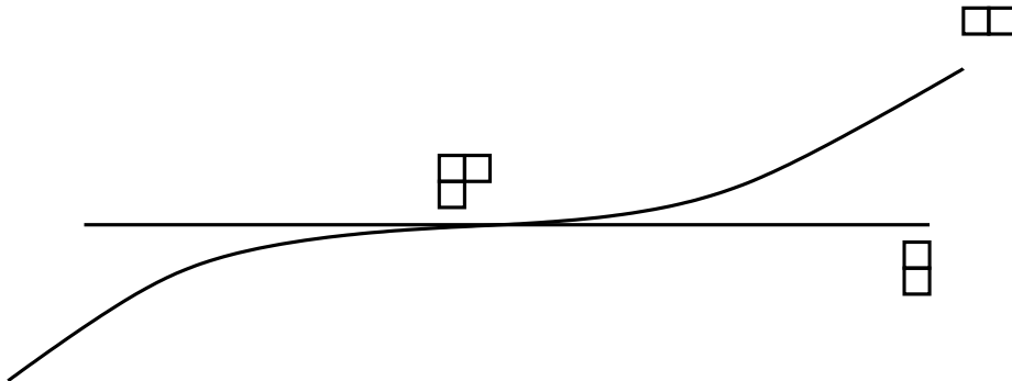
FIGURE 1. One of Kazarian's "generic" bifurcation diagrams. The curves intersect cubically at the origin (like the plane curves of equation y = x^3 and y = 0 at the origin). One of the components corresponds to the curves having a degenerate flattening point of anomaly sequence 2 while for the other component the anomaly sequence is (1, 1) .
