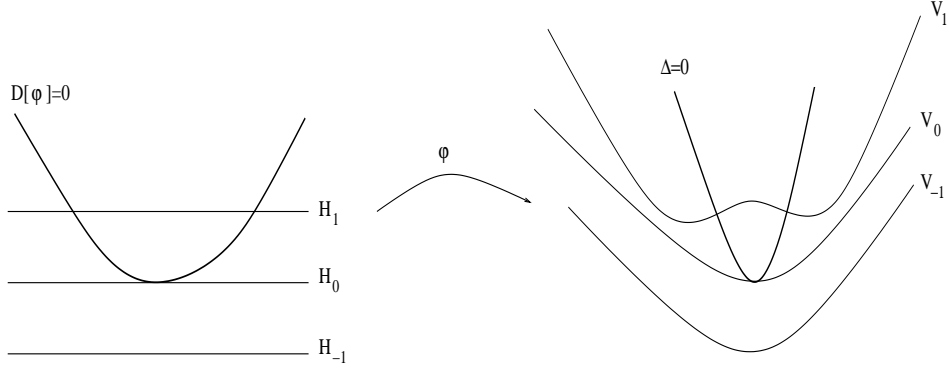
FIGURE 12. The inflection points of V_\varepsilon = \varphi(H_\varepsilon) are the images under \varphi of the intersection points of the curve X = \{(x, y) \in \mathbb{R}^2 : \mathcal{D}[\varphi](x, y) = 0\} with the level-curve H_\varepsilon = \{(x, y) \in \mathbb{R}^2 : H(x, y) = \varepsilon\} . For \varepsilon = 1 the curve V_\varepsilon has two (real) inflection points that coalesce for \varepsilon = 0 . The intersection of the curves H_0 and X at the origin is not transversal.
