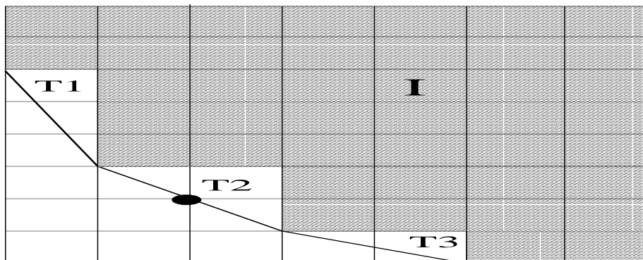
FIGURE 1. The monomial x^2y^2 is the only monomial belonging to the Newton diagram of x^6 + x^3y + xy^3 + y^6 which is not contained in the ideal I . It lies on the hypotenuse of the triangle T2 .
