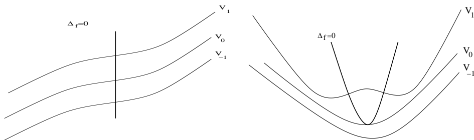
FIGURE 11. Two examples of Hessian curves. The Hessian curve X_f = \{(x, y) : \Delta_f(x, y) = 0\} intersects the curve V_\varepsilon = \{(x, y) : f(x, y) = \varepsilon\} at an inflection point. If the point p is a non-degenerate inflection point then the intersection of V_\varepsilon with X_f at p is transversal (left-hand side).
