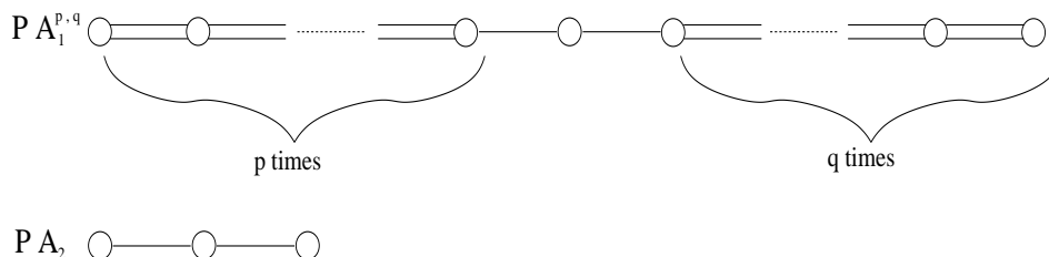
FIGURE 16. Dynkin type diagrams for the \mathcal{P} -fundamental groups of the \mathcal{P} -simple singularities.
