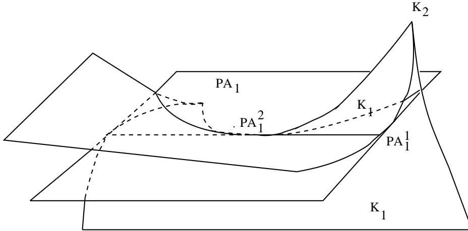
FIGURE 6. The \mathcal{P} -discriminant of the family of curves \mathcal{P}A_1^2 : xy + x^5 + \lambda_1 x^4 + \lambda_2 x^3 + y^3 = \varepsilon . The stratum K_j corresponds to the values of the parameter (\lambda, \varepsilon) for which the curve V_{\lambda, \varepsilon} has a degenerate inflection of anomaly j + 1 . A transversal slice of the surface gives two curves intersecting with multiplicity 4 at the origin.
