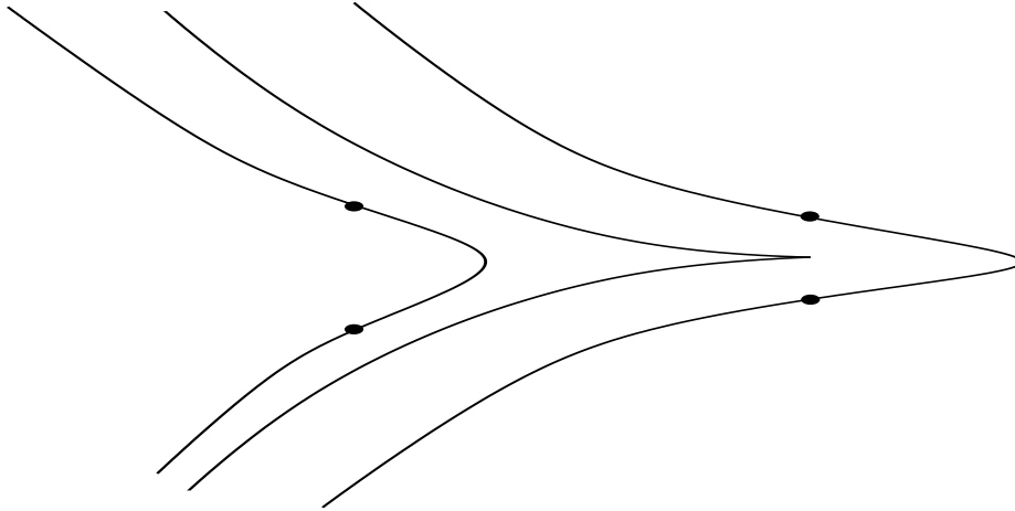
FIGURE 2. The real part of the family of curves V_\varepsilon = \{(x, y) \in \mathbb{C}^2 : y^2 + x^3 = \varepsilon\} for real values of the parameter \varepsilon . Among the 8 complex inflection points of V_\varepsilon , \varepsilon \neq 0 only 2 are real.
