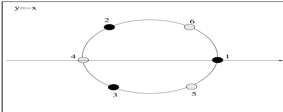
FIGURE 2. Approximated projections of the preinflection points of the curves H_\varepsilon on the y = -x complex-line. The line with an arrow represents the projection for real values of x and y . It contains the two real approximated preinflection points 1 and 4.
