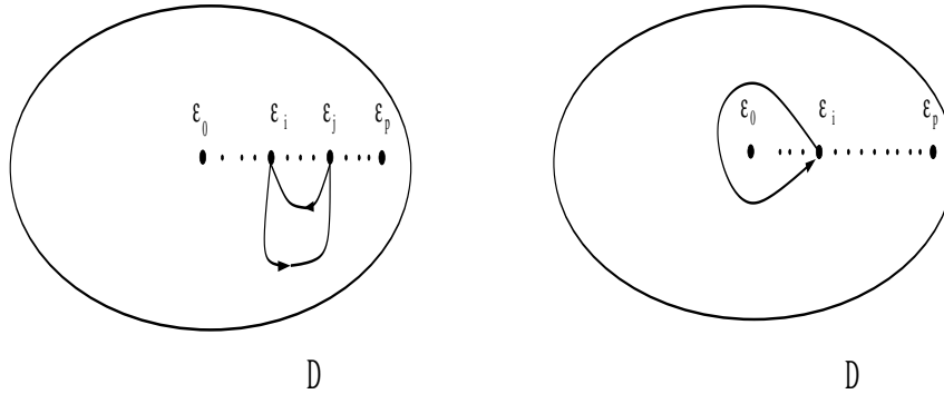
FIGURE 5. The loops \gamma_{j,k} that generate the fundamental group of \mathbb{C}^p \setminus \Sigma .
