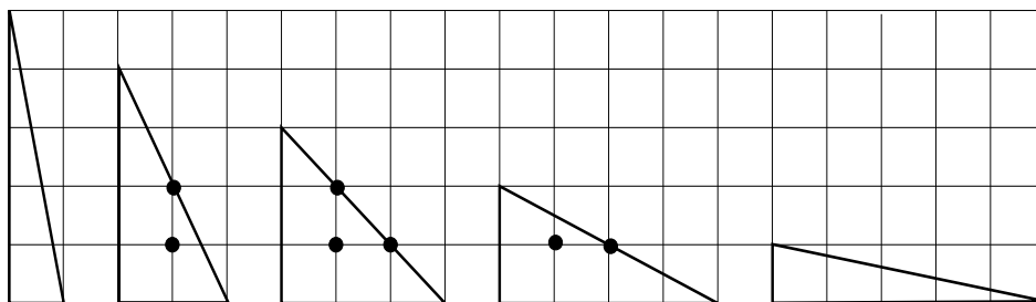
FIGURE 14. Counting a lower bound of the \mathcal{P} -modality by means of combinatorics for the case n = 5 .
