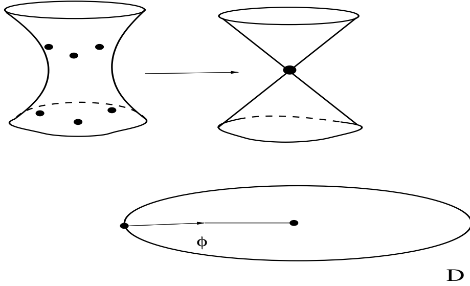
FIGURE 15. Vanishing inflection points at a generic Morse critical point of a holomorphic function f from the topological view-point (compare with figure 1 of page 18). The complex curve of equation f = \varepsilon is locally homeomorphic to a cylinder provided that \varepsilon \neq 0 . The inflection points are 6 marked points on the cylinder. When \varepsilon goes to zero the 6 points converge towards the singular point of the cone.
