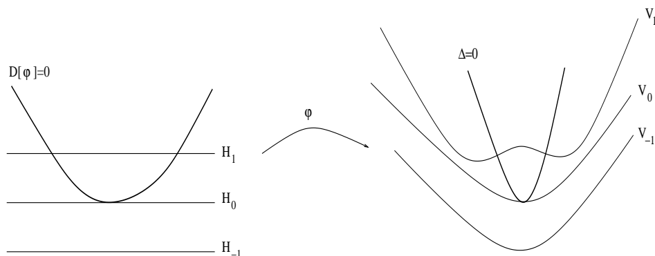
FIGURE 2. The inflection points of V_\varepsilon are the images under \varphi of the intersection points of the curve X = \{(x, y) \in \mathbb{C}^2 : \mathcal{D}[\varphi](x, y) = 0\} with H_\varepsilon = \{(x, y) \in \mathbb{C}^2 : H(x, y) = \varepsilon\} . For \varepsilon = 1 the curve V_\varepsilon has two real inflection points that coalesce for \varepsilon = 0 . The intersection of the curves H_0 and X at the origin is not transversal.
