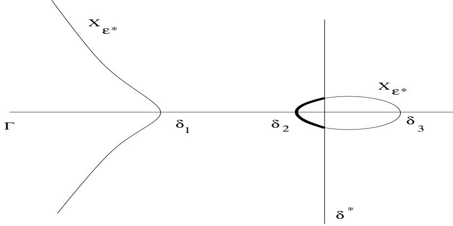
FIGURE 4. We have drawn the real part of a complex curve (in fact an elliptic curve in this case) X_{\varepsilon^*} for \varepsilon^* \in \mathbb{R} . The restriction g of the linear function l : (x, y) \mapsto x to X_{\varepsilon^*} has three critical points of critical values \delta_1, \delta_2, \delta_3 . The bolded part of the oval is the pre-image under g of \delta_2 . It defines a relative one-dimensional cycle associated to \delta_2 . The other half of the oval is the pre-image under g of \delta_3 . The relative cycle associated to \delta_1 passes through the complex domain.
