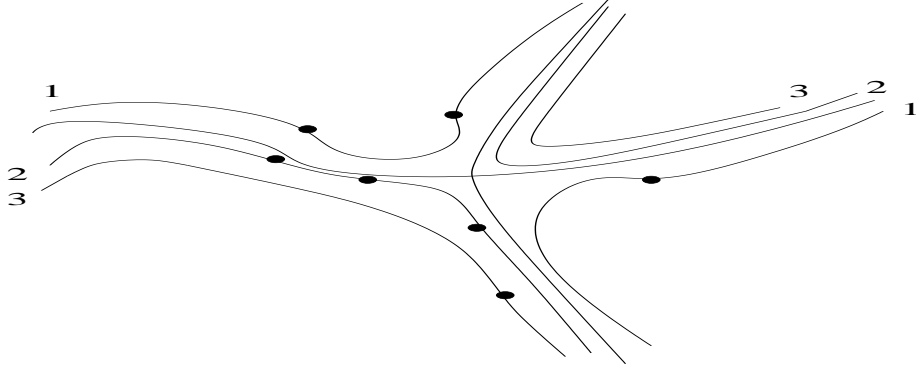
FIGURE 5. We have numbered the level curves in \mathbb{R}^2 by 1, 2, 3. The black disks stand for the inflection points of the curves labelled 1, 2, 3. The number 1 curve and the number 2 curve have 3 (real) inflection points. The number 3 curve has only one real inflection point. Between the curve 2 and the curve 3 there is a curve with a degenerate inflection point. Between 1 and 2 there is a curve with a node singular point. This singular curve has an inflection point.
