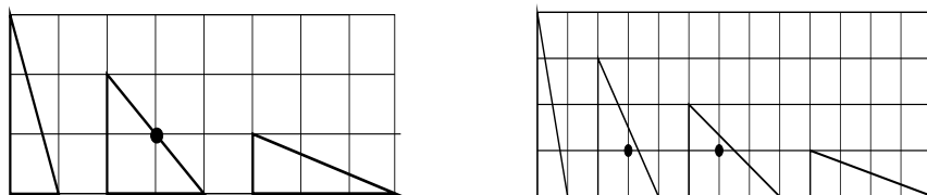
FIGURE 13. Counting a lower bound of the \mathcal{P} -modality by means of combinatorics for the cases n = 3 and n = 4 .
