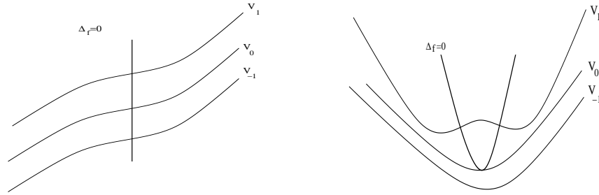
FIGURE 1. Two examples of Hessian curves. At a non-degenerate inflection point the Hessian curve intersects transversally the level curve (left part).
