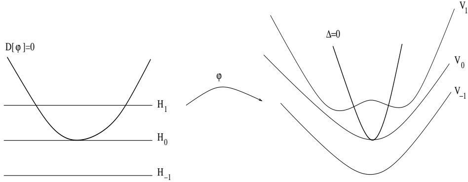
FIGURE 2. For \varepsilon = 1 the curve V_1 has two real inflection points that coalesce when \varepsilon \rightarrow 0 .
