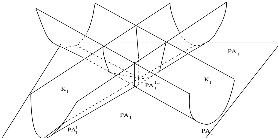
FIGURE 8. The \mathcal{P} -discriminant of the family of curves \mathcal{P}A_1^{1,1,+} : xy + x^4 + y^4 + \lambda_1 x^3 + \lambda_2 y^3 = \varepsilon . The stratum K_j corresponds to the values of the parameter (\lambda, \varepsilon) for which the curve V_{\lambda, \varepsilon} has a degenerate inflection point of anomaly j + 1 .
