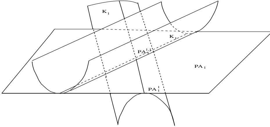
FIGURE 9. the \mathcal{P} -discriminant of the family of curves \mathcal{P}A_1^{1,1,-} : xy + x^4 - y^4 + \lambda_1 x^3 + \lambda_2 y^3 = \varepsilon . The stratum K_j corresponds to the values of the parameter (\lambda, \varepsilon) for which the curve V_{\lambda, \varepsilon} has a degenerate inflection point of anomaly j + 1 .
