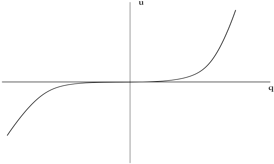
FIGURE 4. The wave front of the Legendre variety generated by F(q, u, t) = 2t^3 - 3qt^2 + u . It has two branches: the q -axis and a smooth curve cubically tangent to it.
