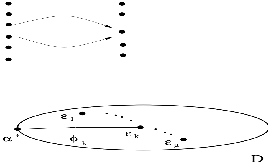
FIGURE 1. Zero-dimensional vanishing cycle at a Morse critical point. When \varepsilon approaches a critical value of a Morse critical point of f two preimages coalesce.
