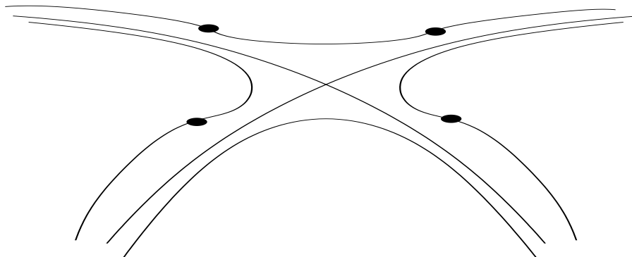
FIGURE 1. Vanishing inflection points at a generic Morse critical point of a real analytic function f . We have drawn the level curves f = \varepsilon in the affine plane \mathbb{R}^2 . The complexification of the level curve f = \varepsilon is a Riemann surface with 6 inflection points. Among the six inflection points of this complex holomorphic curve no more than two can be real. The two inflection points of the real curve of equation f = \varepsilon lie either on two distinct components or on the same component (depending on the sign of \varepsilon ).
