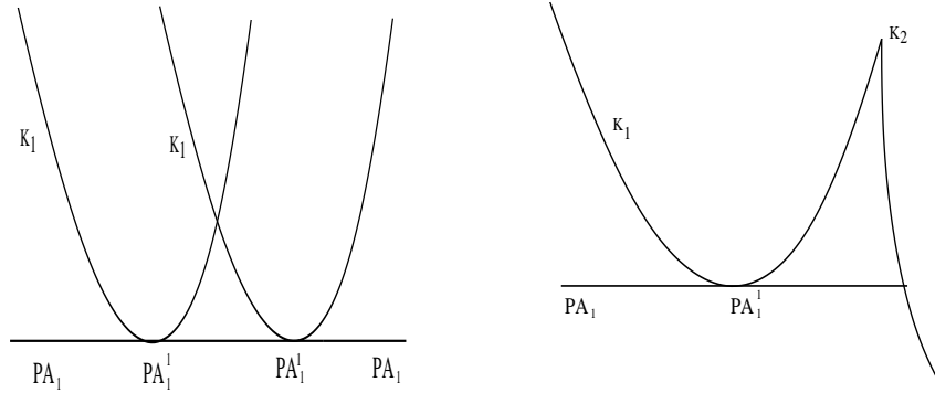
FIGURE 10. Left-hand side: plane section of the \mathcal{P} -discriminant \mathcal{P}A_1^{1,1,+} . Right-hand side: plane section of the \mathcal{P} -discriminant \mathcal{P}A_1^2 . The stratum K_j corresponds to the values of the parameter (\lambda, \varepsilon) for which the curve V_{\lambda, \varepsilon} has a degenerate inflection point of anomaly j + 1 .
