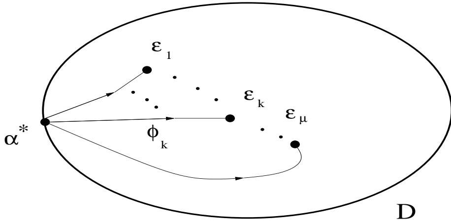
FIGURE 3. A distinguished basis.
