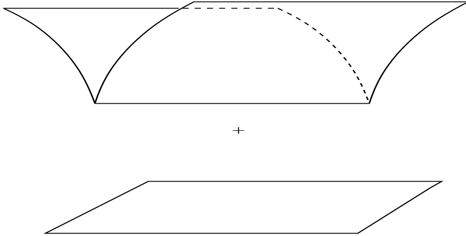
FIGURE 7. One component of the \mathcal{P} -discriminant of \mathcal{P}A_1^2 is diffeomorphic to a cylinder over a semi-cubical parabola. The other component is a plane.
