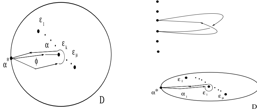
FIGURE 2. On the left hand side: the closed loop \alpha associated to the path \phi . On the right hand side: the monodromy associated to the loop \alpha .
