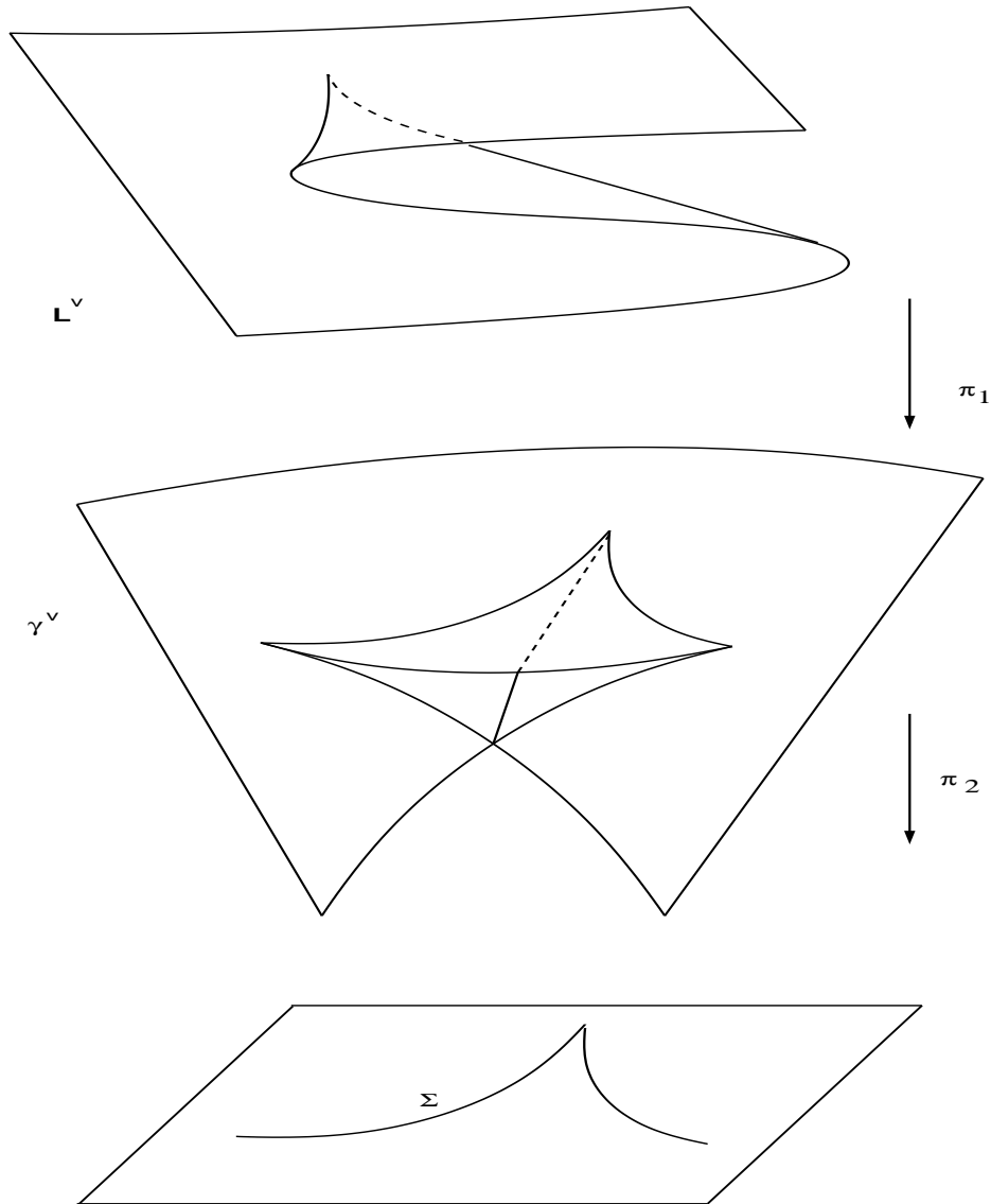
FIGURE 5. The Legendrian projection corresponding to a non-degenerate flattening point of a space curve.
