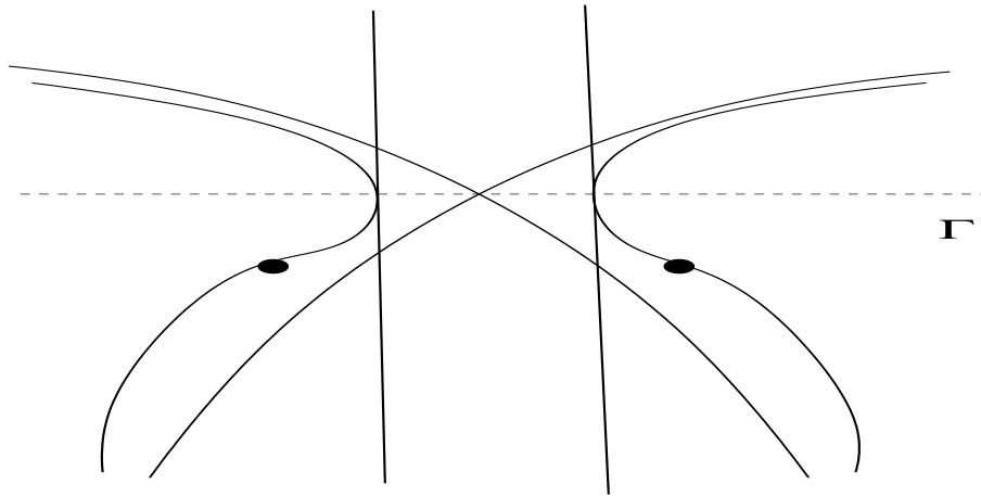
FIGURE 3. There are two vanishing tangent lines at a node singular point. The polar curve \Gamma intersects the singular curve with multiplicity equal to two at the singular point.
