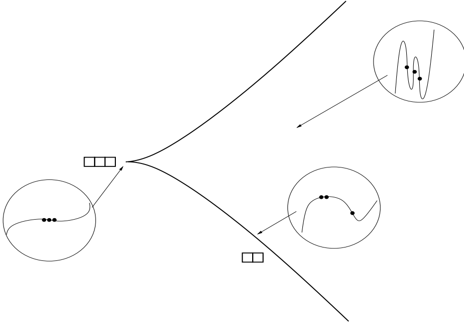
FIGURE 3. The \mathcal{P} -discriminant of the family of curves (V_\lambda) given by V_\lambda = \{(x, y) \in \mathbb{R}^2 : y + x^5 + \lambda_1 x^3 + \lambda_2 x^2 = 0\} . Inside the disks, we represented the real parts of the curve of the corresponding value of the parameter. The marked points on the curves stand for the inflection points. In case of a degenerate inflection point, we have put the marked points near one to the other.
