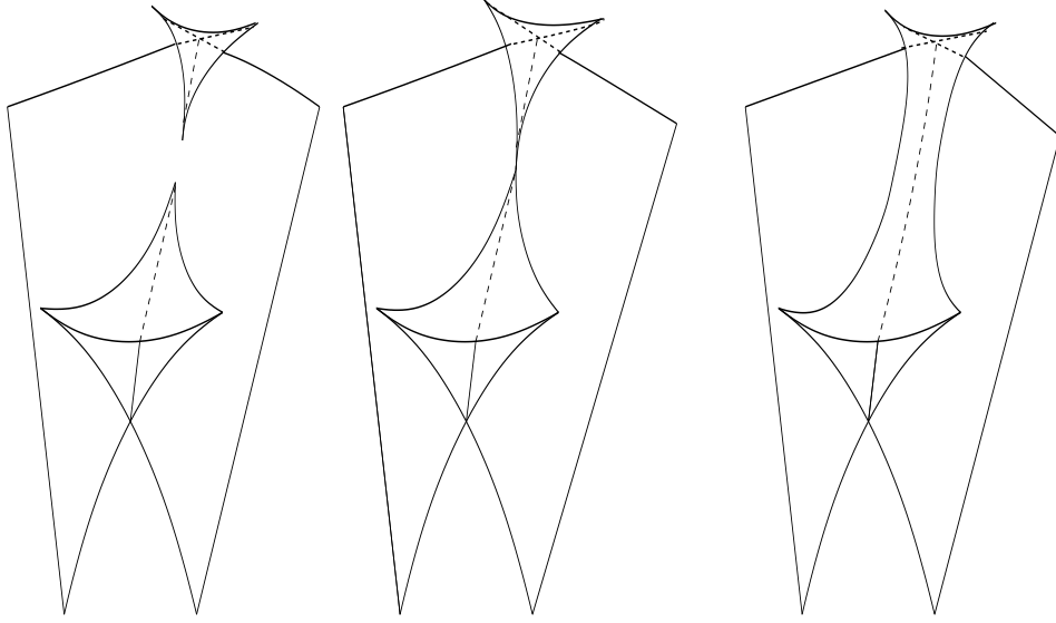
FIGURE 6. A "typical" bifurcation of wave-fronts.
