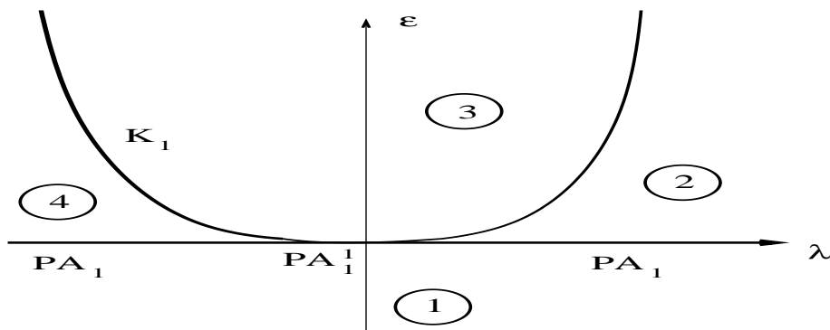
FIGURE 4. The real \mathcal{P} -discriminant of the function F(\lambda, x, y) = xy + x^4 + \lambda x^3 + y^3 . The curves corresponding to values of the parameter (\lambda, \varepsilon) in the connected components 1, 2, 3 are depicted in figure 5. The stratum K_1 corresponds to the values of the parameter (\lambda, \varepsilon) for which the curve V_{\lambda, \varepsilon} has a degenerate inflection point of anomaly 2. The values of the parameters (\lambda, \varepsilon) for which the curve V_{\lambda, \varepsilon} is singular has two strata. One stratum of dimension 1 denoted \mathcal{P}A_1 and a stratum of dimension 0 denoted \mathcal{P}A_1^1 which lies in the closure of the the strata of dimension 1. The stratum \mathcal{P}A_1 is not connected (while in the complex case it is connected).
