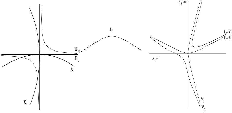
FIGURE 1. The Plücker theorem. In the right part of the figure among the 6 inflection points of a curve V_\varepsilon = \varphi(H_\varepsilon) only 2 have real coordinates (for a real value of the parameter \varepsilon ). The preimages of the inflection points of V_\varepsilon under \varphi are the intersection points of the curve H_\varepsilon with the curve X = \{(x, y) \in \mathbb{C}^2 : \mathcal{D}[\varphi](x, y) = 0\} .
