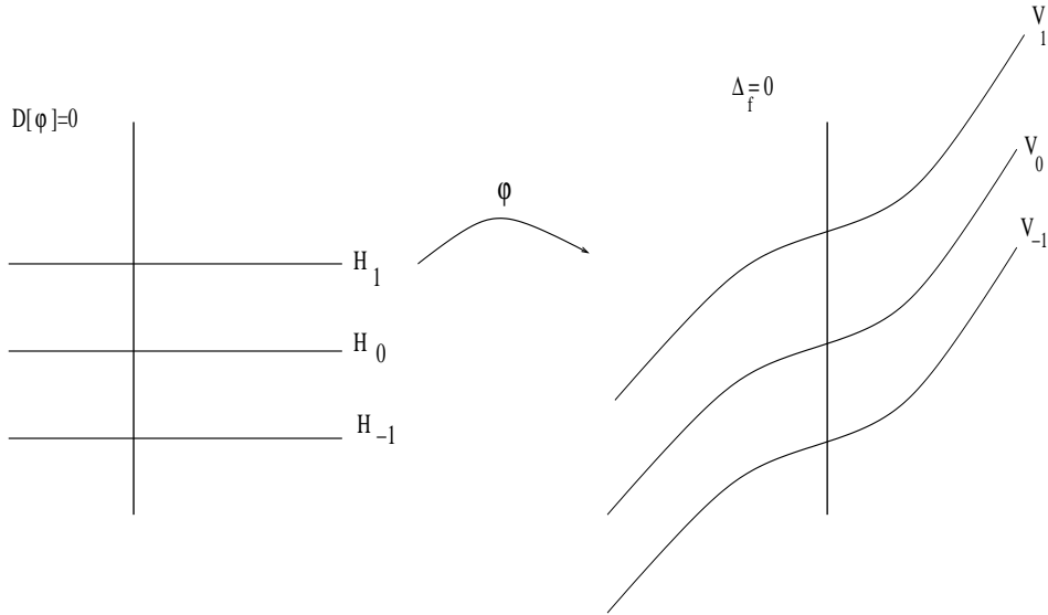
FIGURE 1. In the left hand-side the intersection points of the curves of equations y = \varepsilon, x = 0 correspond to inflection points of the curves V_\varepsilon \subset \mathbb{C}^2 in the right hand-side.
